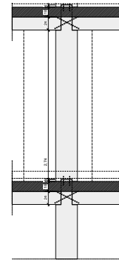
Detail of floor-wall connection. Detail credit: Rozynski Sturm Architekten
