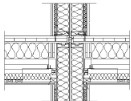
Detail showing a connection between interior wall and floor; the wall and floor elements are discontinuous at the joint.
