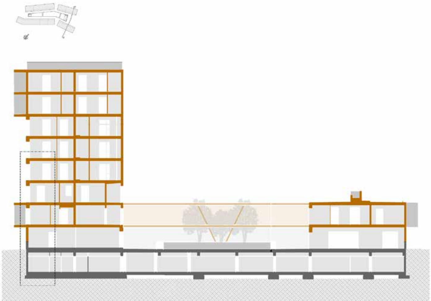
Elevation view. Detail Credit: ROSSIPRODI ASSOCIATI srl.
