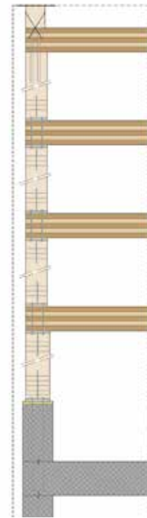
Schematic of Floor and Wall panels. Detail Credit: ROSSIPRODI ASSOCIATI srl.
