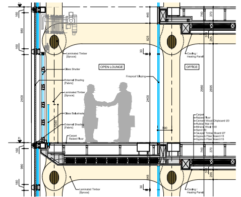
Detail of raised floor and exterior glazing Detail Credit: Shigeru Ban Architects
