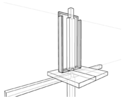
Interlocking wood structure Detail credit: Rozynski Sturm Architekten
