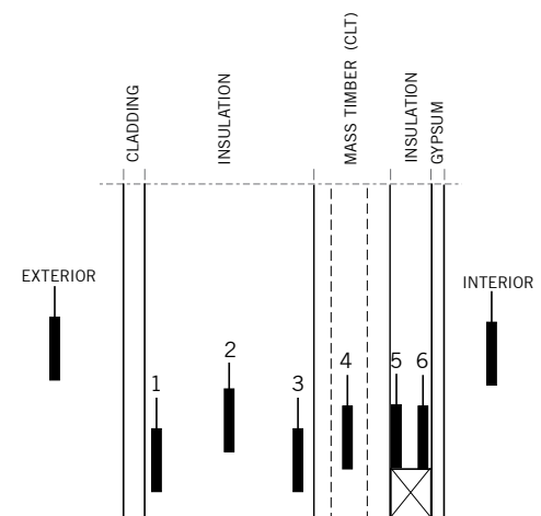
Location of moisture sensors. Detail Credit: Outstanding
