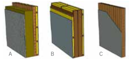
A) Exterior wall B) Separation wall C) Partition Wall
