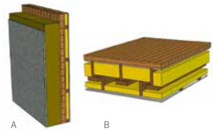
A) 3-ply CLT floor slab strengthened with T-shaped glulam beams.
