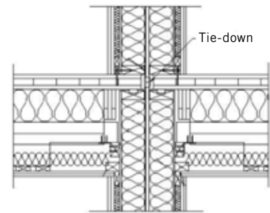
Location of tension rod through the interior wall and floor to assist with stabilization.
