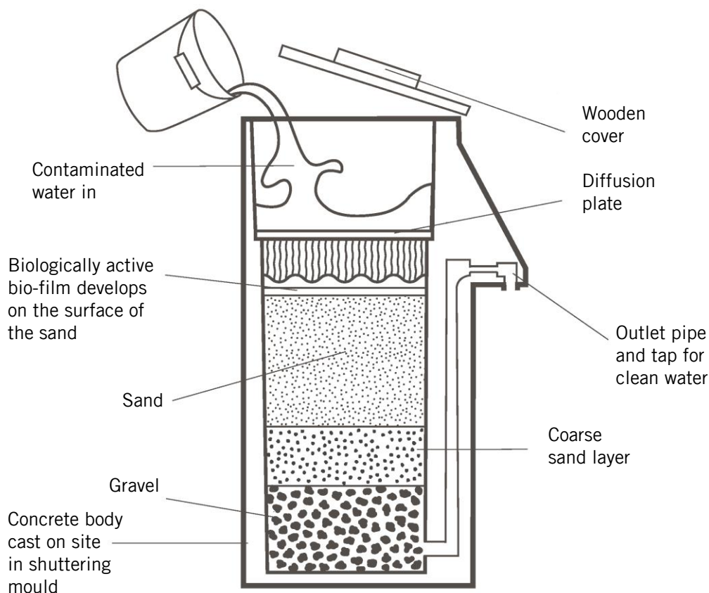
Figure 4: Bio-sand filter cross section.
