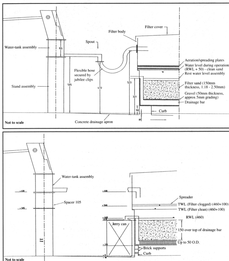
Figure 1. (top) The existing handpump/Mark 1 iron-filter arrangement in use at Lyantonde. Figure 2. (below) The research team's proposed handpump-filter arrangement.
