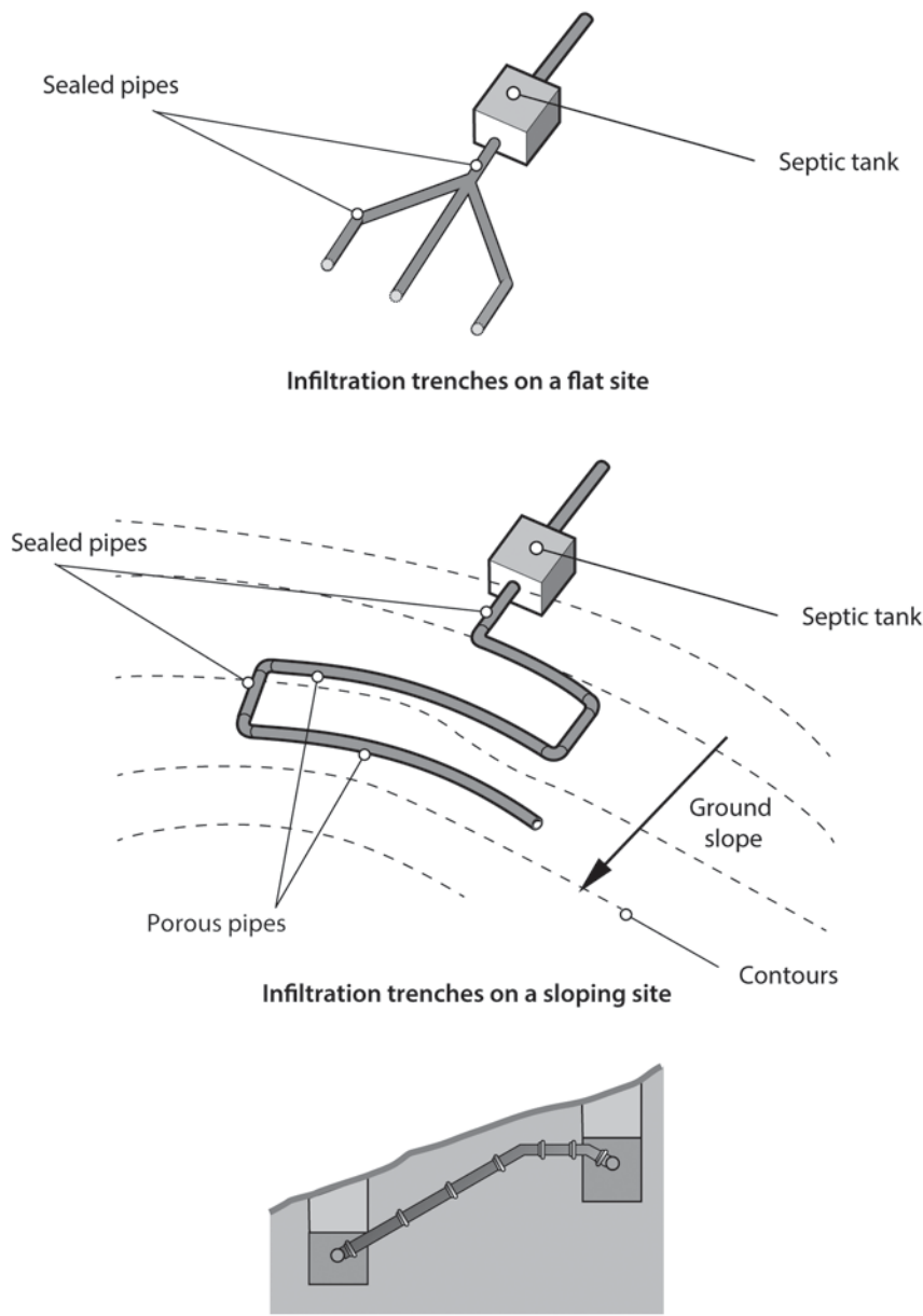
Connection between two infiltration trenches at different levels Figure 10.3 Infiltration trenches
