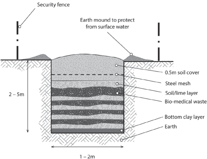
Figure 15.8 Temporary sharps pit
