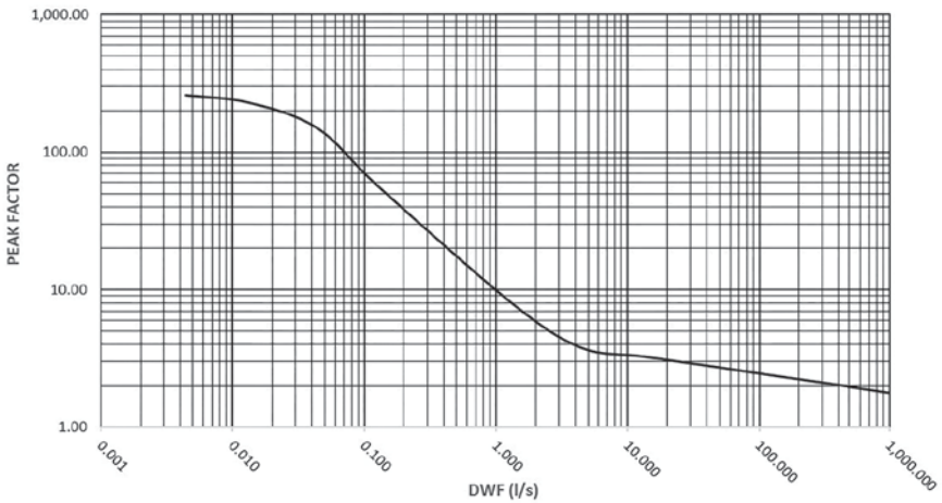
Figure A4.2 Peak factors for very low flows Source: Adapted from (Haws, n.d.)
