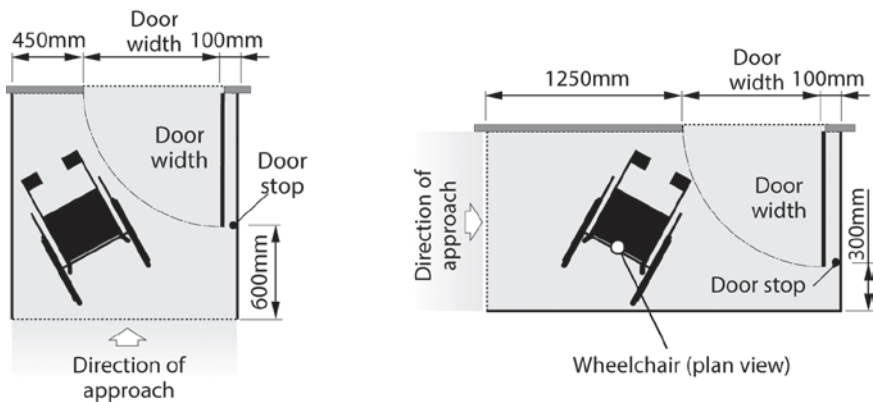
Figure 5.2 Minimum dimensions of the flat platform for opening the toilet door Source: Adapted from (** Jones & Reed, 2005)
