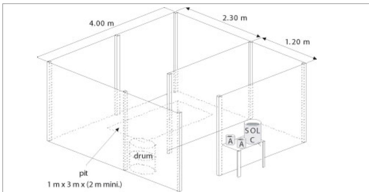
Figure 14.7: Example of excreta-disposal pit.
