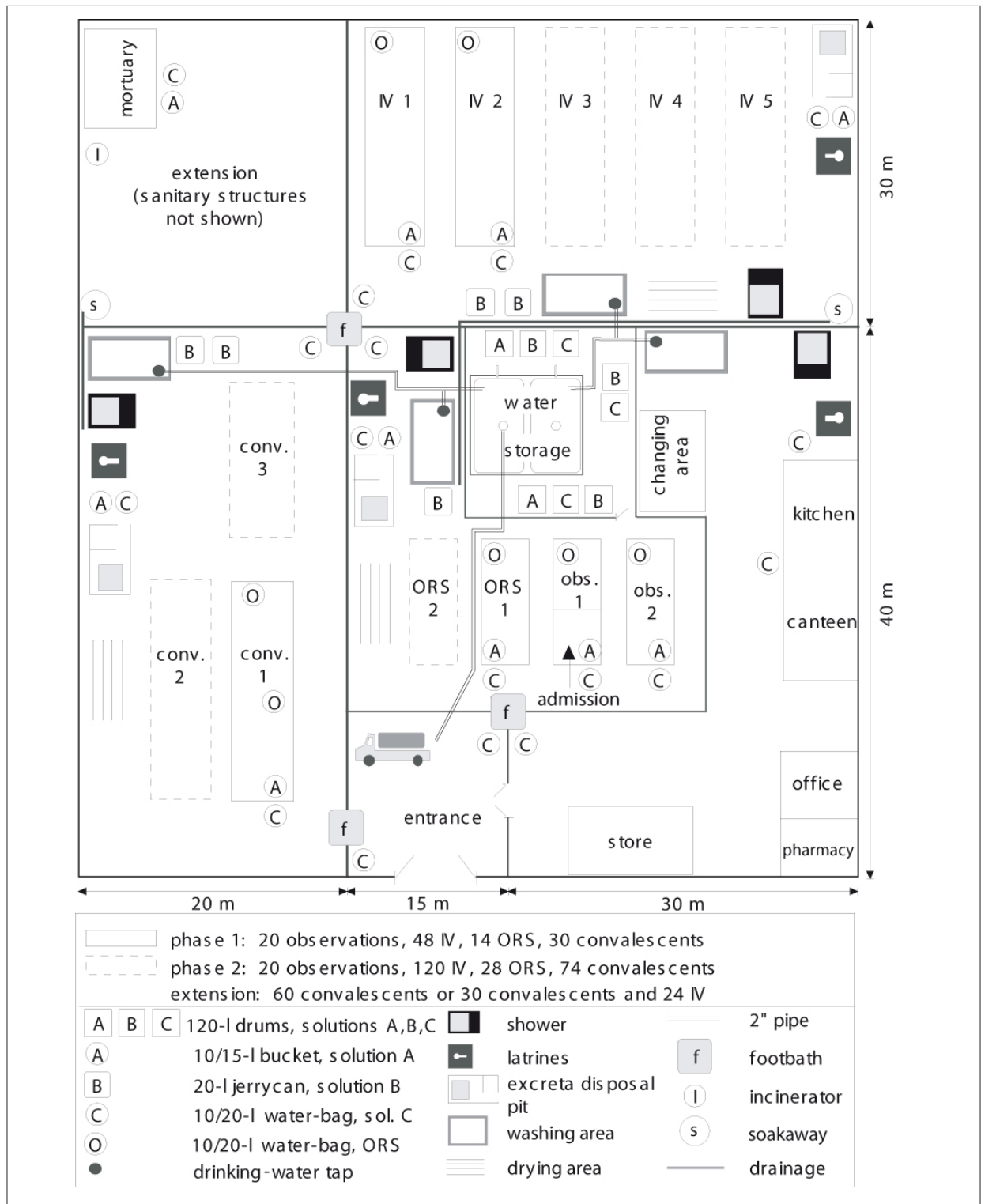
Figure 14.5: Plan of a typical CTC for 300 patients.
