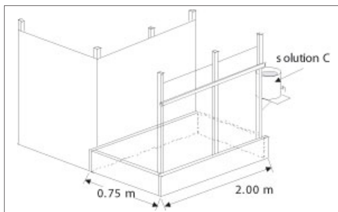
Figure 14.6: Footbath and hand-washing facility.
