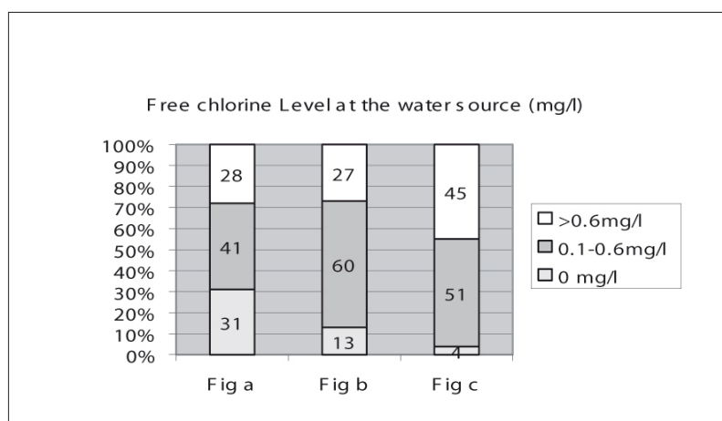
Figure 14.9: Comparative performance of different well-chlorination techniques.
