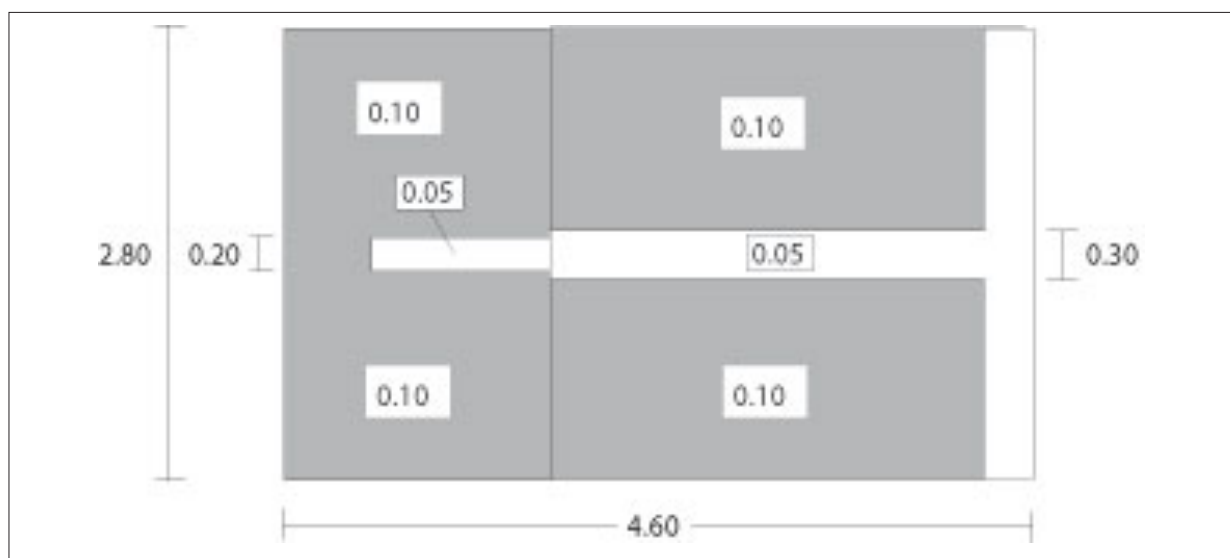
Figure 10.11: Plan of the slab.
