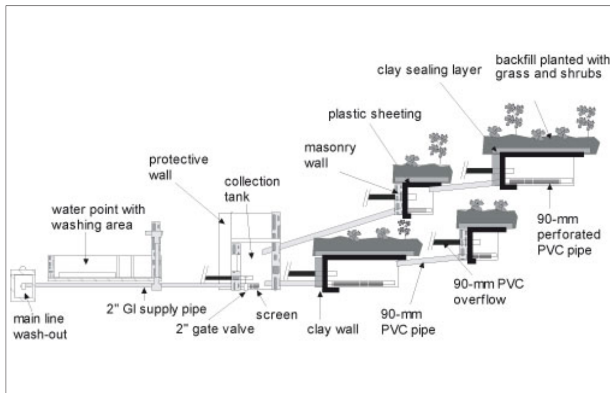
Figure 10.8: Spring catchment.
