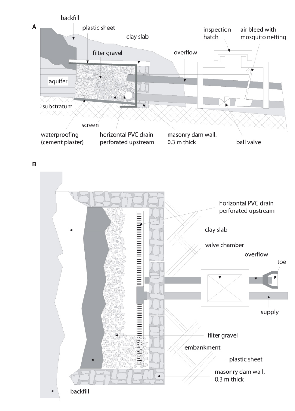
Figure 10.2: Infiltration gallery. A: section. B: plan.
