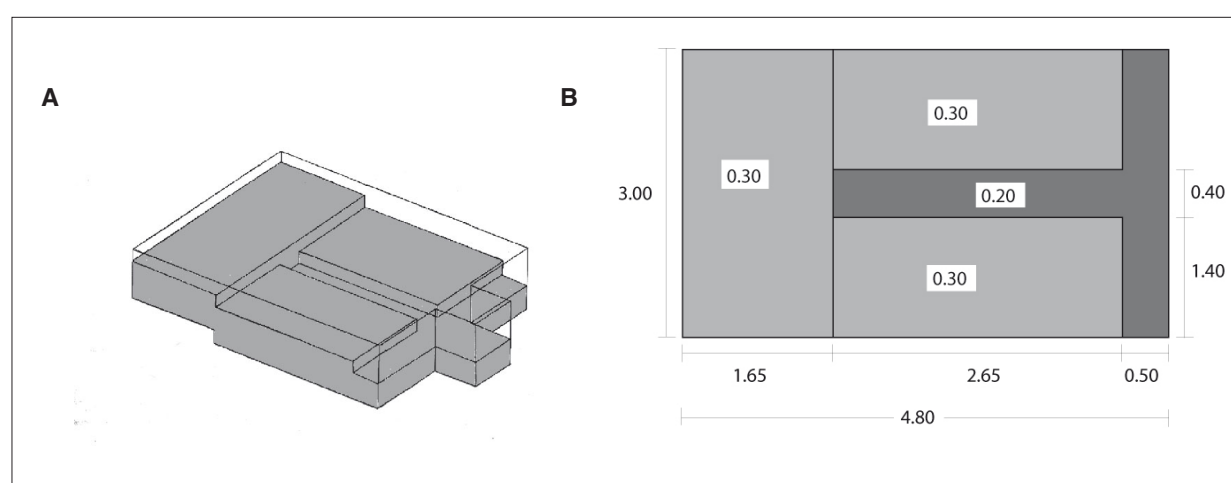
Figure 10.9: Foundations of tapstand and laundry area.
