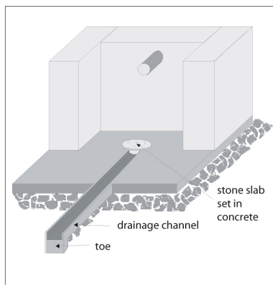
Figure 10.4: Examples of water points. A: simple water point (ACF, Burundi, 1995).
