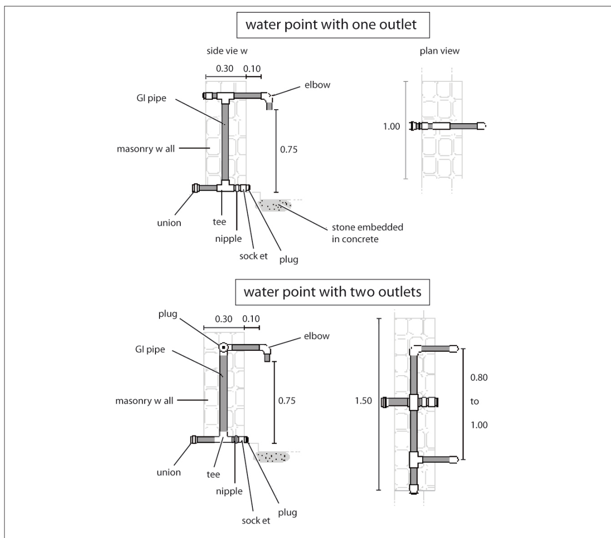
Figure 10.13: Plumbing for water point.
