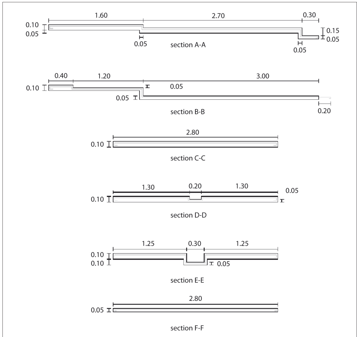
Figure 10.12: Sections of the slab.
