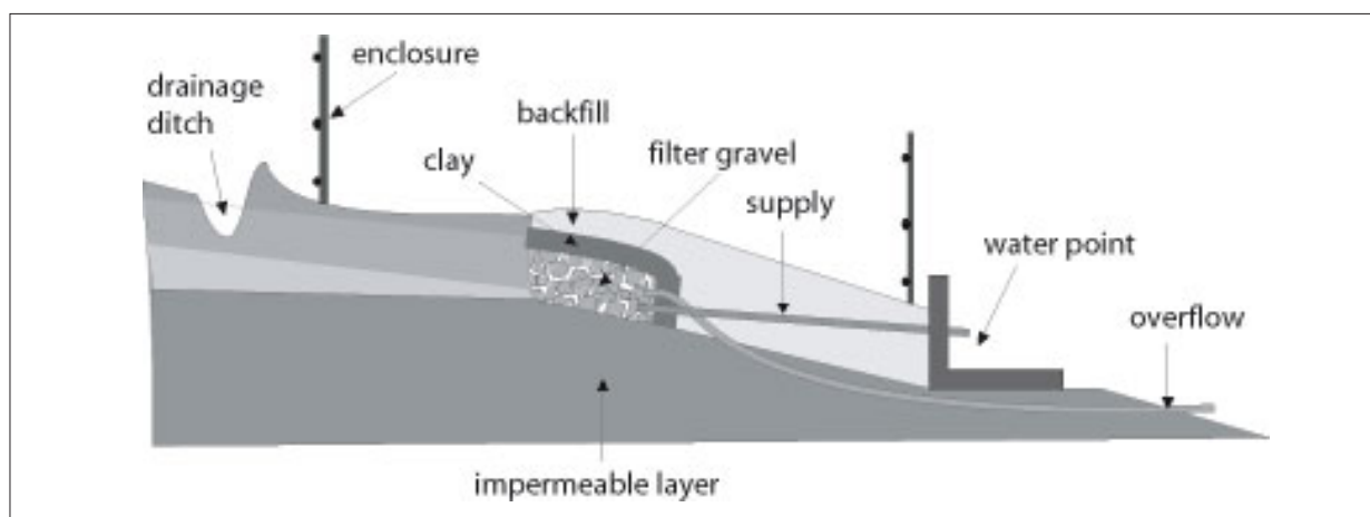
Figure 10.3: Infiltration gallery sealed with clay.
