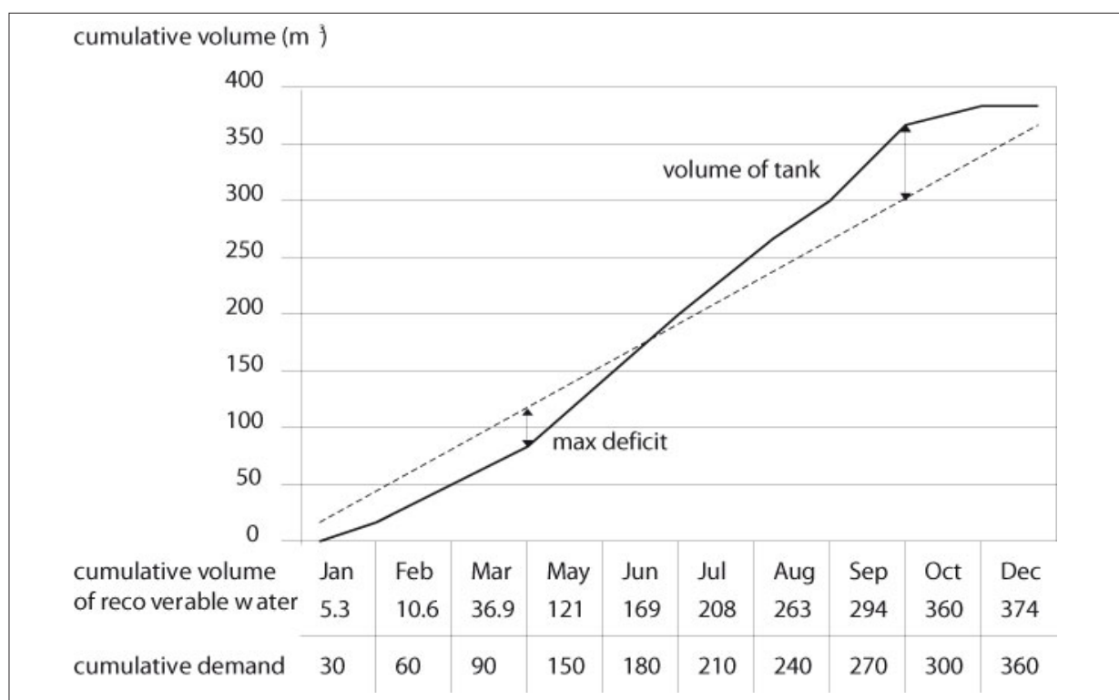
Figure 10.7: Design of a rainwater-catchment tank for a school (ACF, Uganda, 1996).
