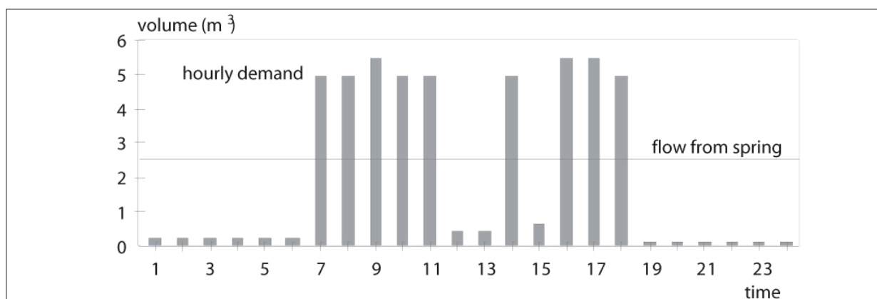
Fig 10.5: Hourly demand vs. flow from a spring.
