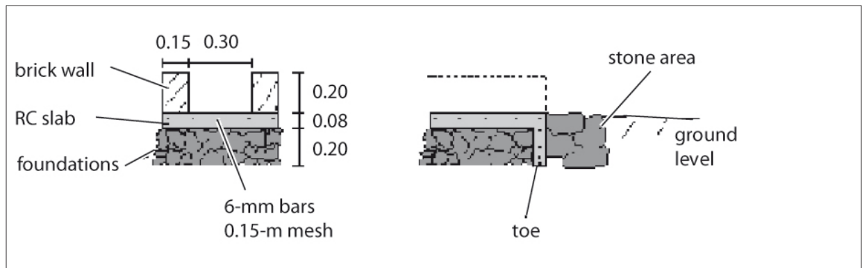
Figure 10.15: Drainage channel (A) and toe (B).
