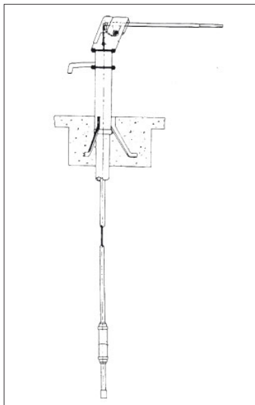
Figure 9.29: India Mark II pumps.
