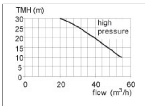
Figure 9.16: Characteristic curve for an electric dewatering pump.
