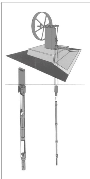
Figure 9.31: Volanta handpump.
