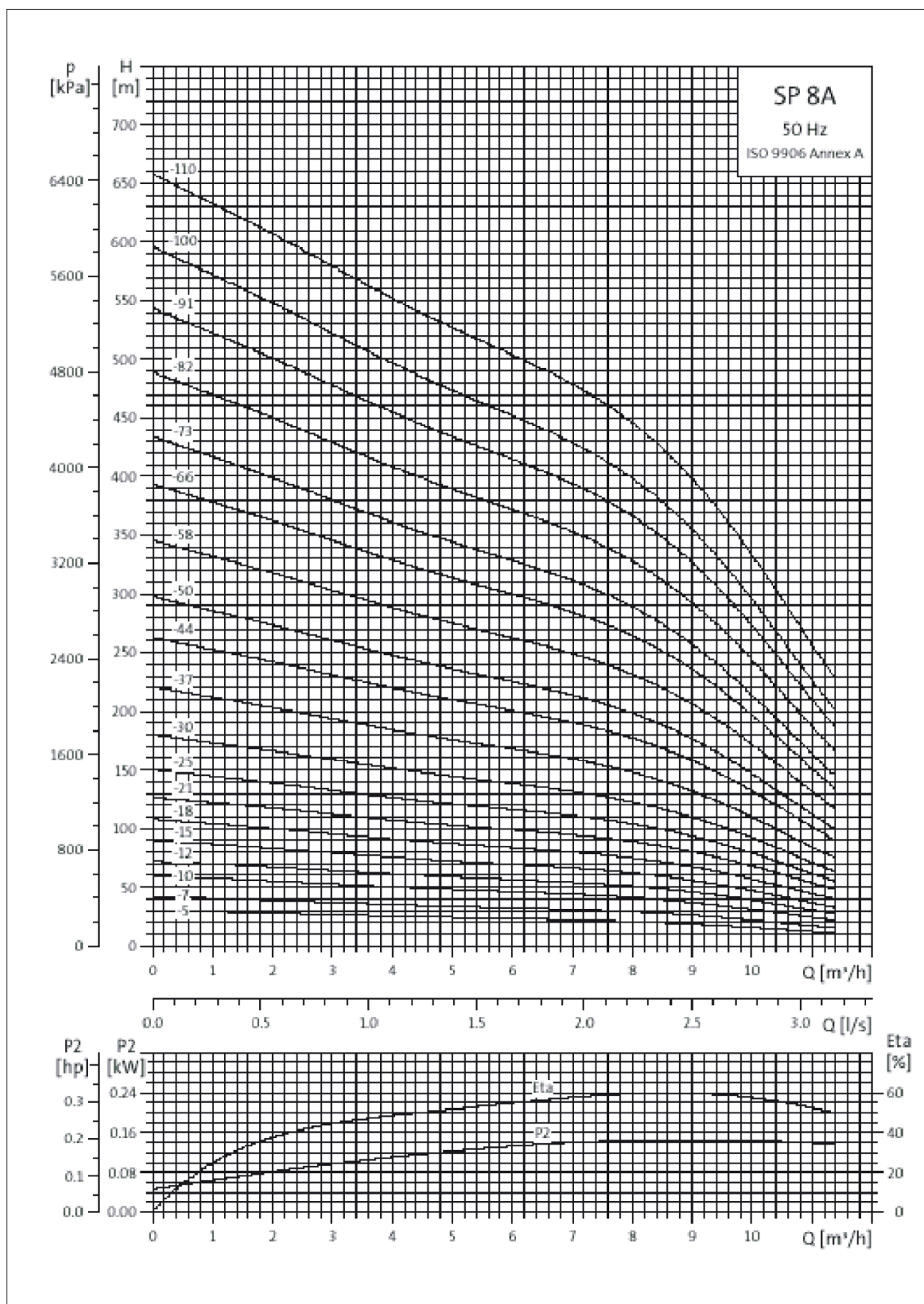
Figure 9.5: Characteristic curve for the Grundfos SP8A range of pumps, and efficiency curves where Q = flow, H = TMH, and \eta = efficiency.
