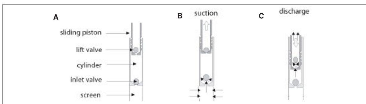
Figure 9.25: Working principle of a piston pump.
