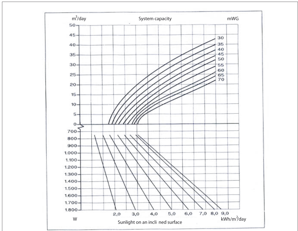
Figure 9.21: Design chart for SP3A-10 pump for 11 hours of sunshine per day and average temperature of 30°C.
