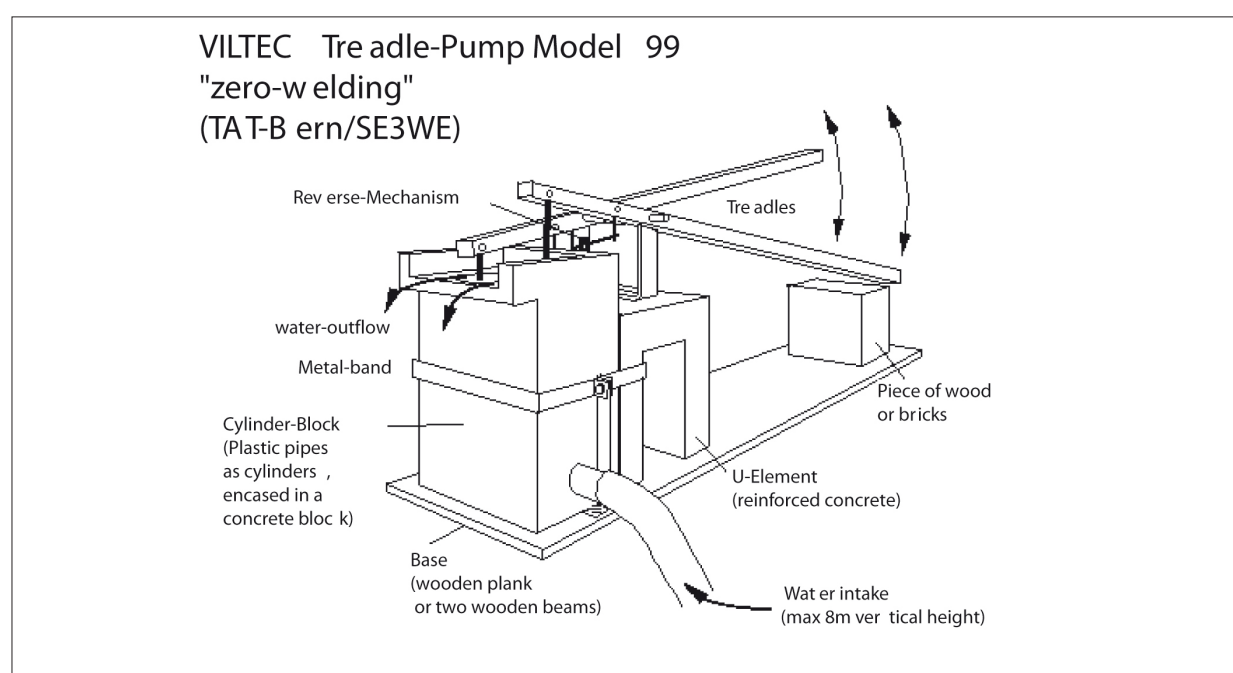
Figure 9.39: Treadle pump (Viltec treadle-pump model 99 “zero welding”).
