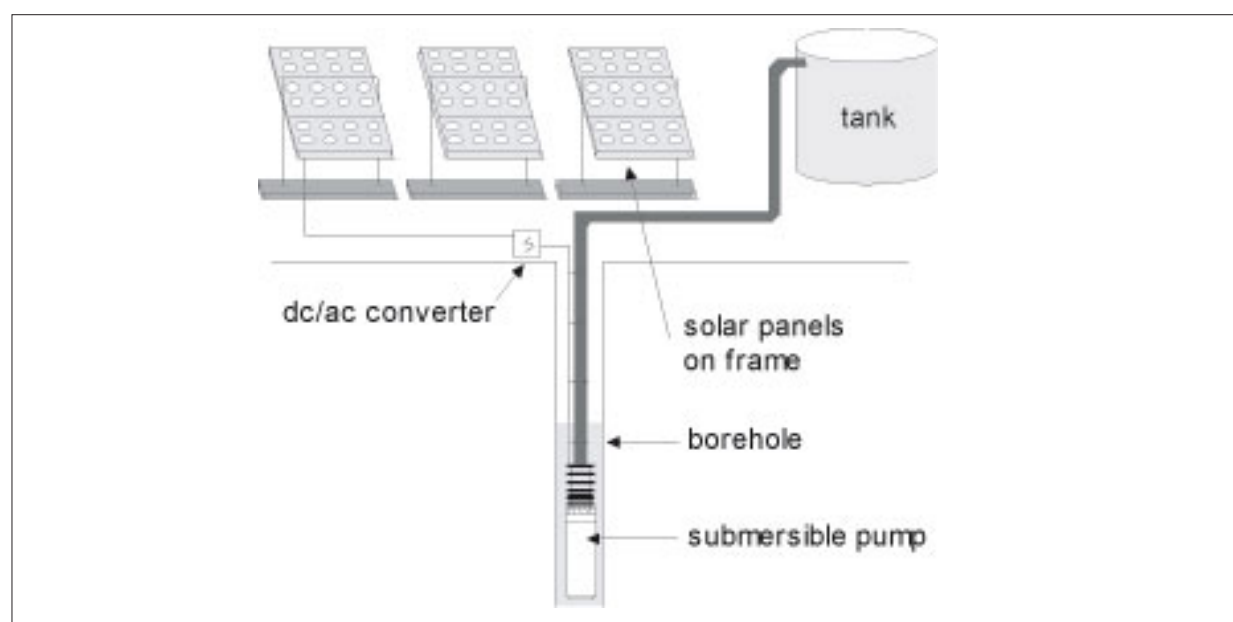
Figure 9.20: Supplying a pump using solar panels.
