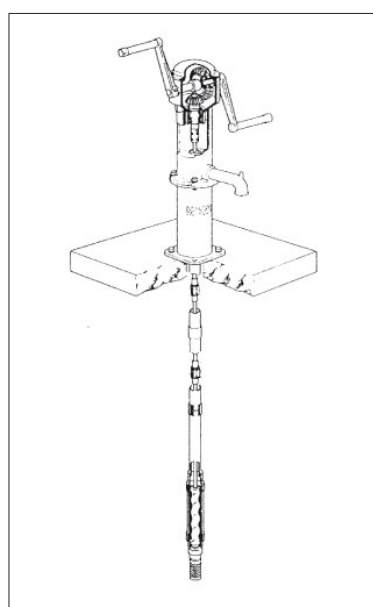
Figure 9.36: Pumping to a tank using a Monolift pump.
