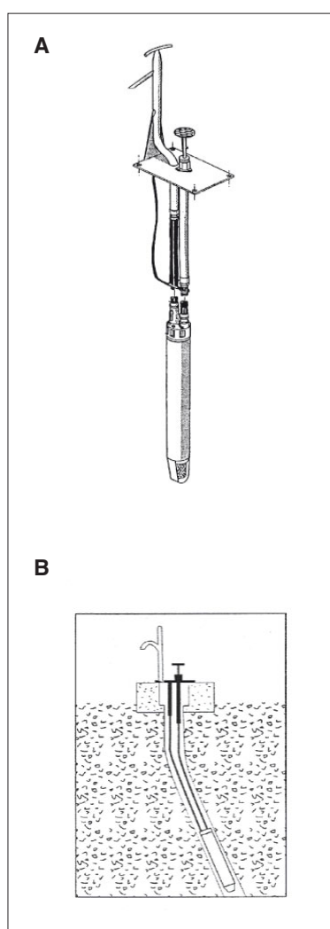
Figure 9.33: Working principle of Vergnet hydropump.
