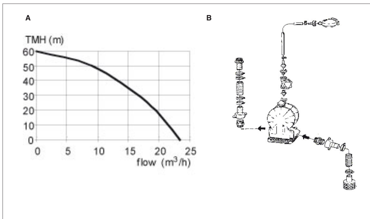
Figure 9.19: Membrane dewatering pump.
