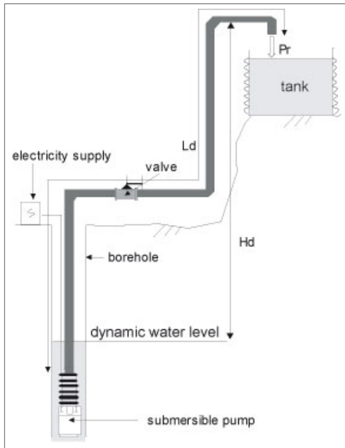
Figure 9.14: Installation plan for a submerged multistage electric pump.
