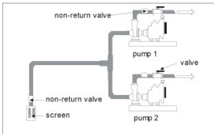
Figure 9.10: Mounting two pumps in parallel.
