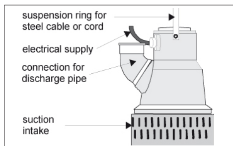
Figure 9.17: Electric dewatering pump. Model 2102 HT 234; weight: 50 kg; height and diameter: 660 x 470 mm; discharge diameter: 2"; nominal power: 4.6 kW; supply voltage: 380 V, 50 Hz three-phase or 220 V, 50 Hz three-phase
