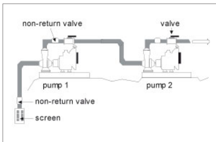
Figure 9.8: Mounting two identical pumps in series.
