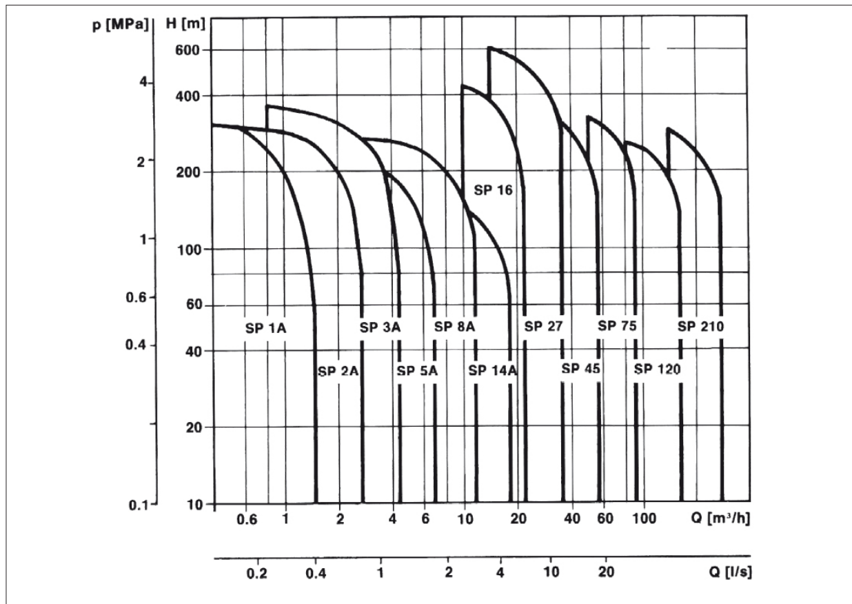
Figure 9.15: Range of Grundfos pumps.
