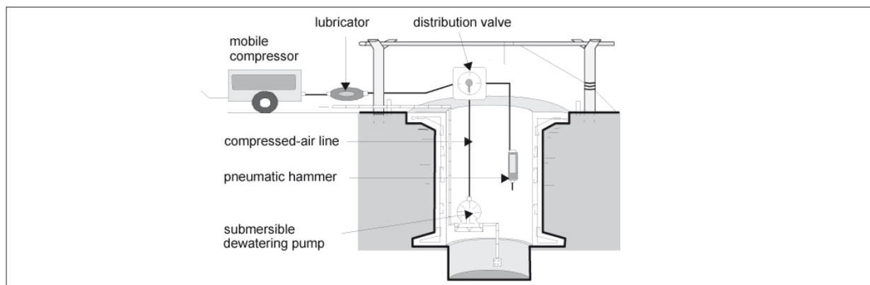
Figure 9.18: Using a pneumatic pump and a pneumatic hammer in well digging.
