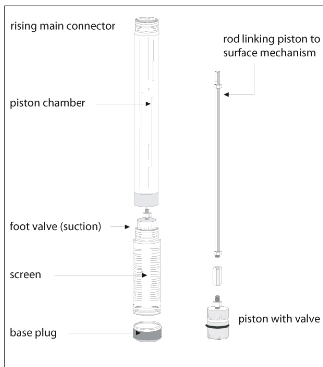
Figure 9.27: Kardia pump cylinder.
