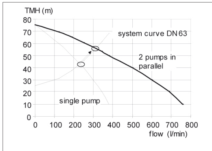
Figure 9.11: Characteristic curves for two pumps mounted in parallel.
