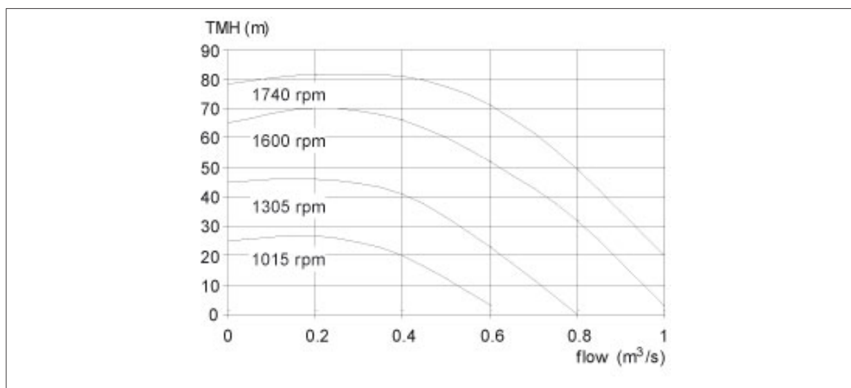
Figure 9.7: Characteristic curves for a centrifugal pump as a function of rotational speed.
