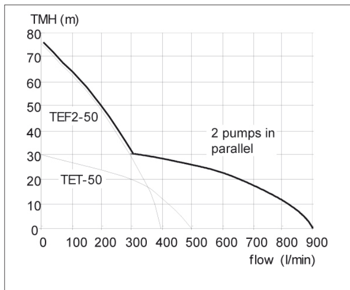
Figure 9.12: Characteristic curves for two different pumps in parallel (types TET-50 and TEF2-50).
