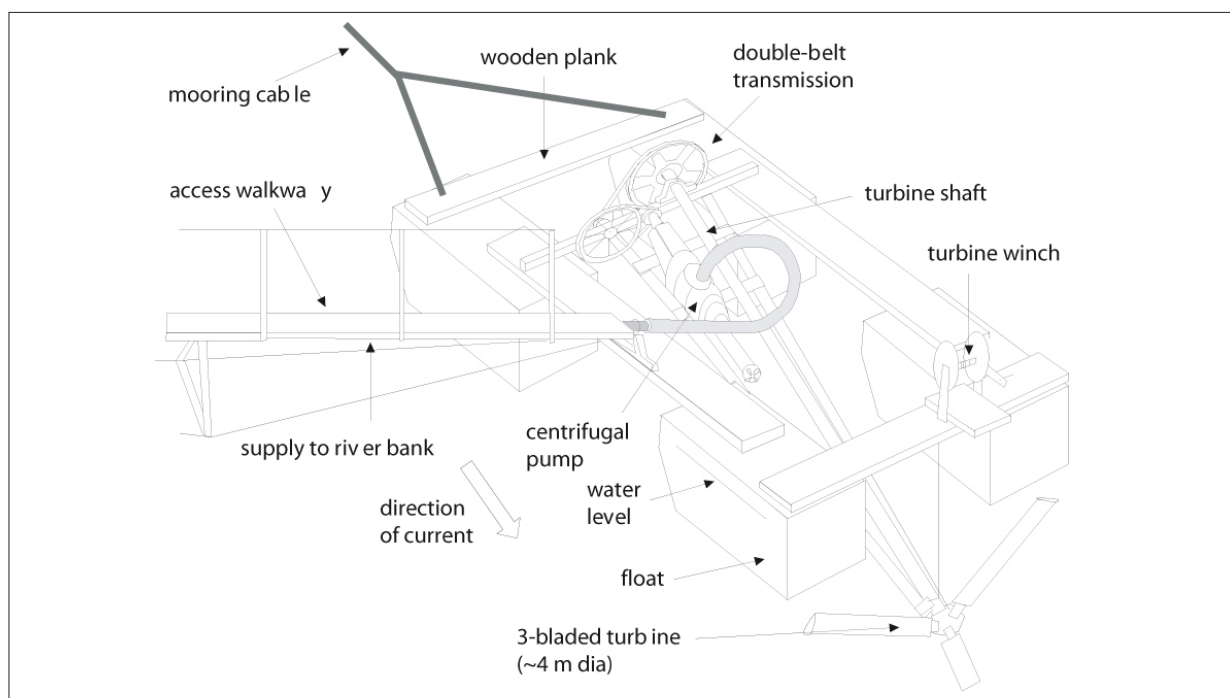
Figure 9.22: Garman pump installed on a raft.
