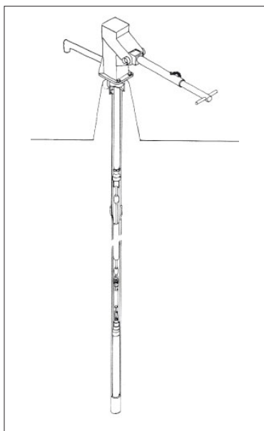
Figure 9.30: Aquadev and Afridev pumps.
