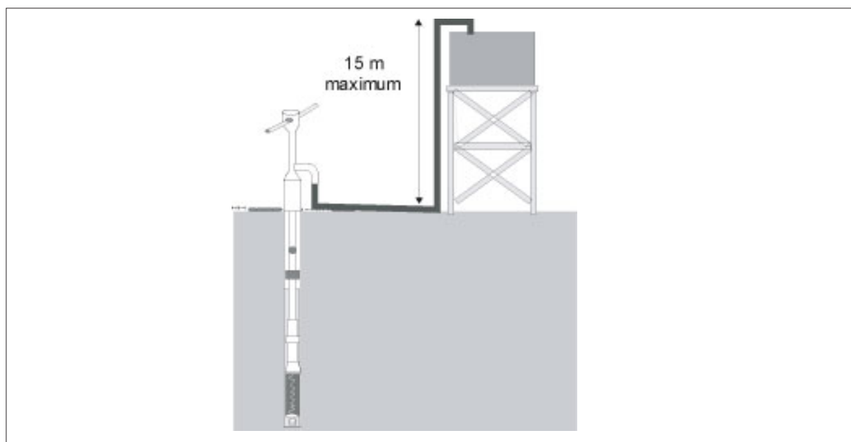
Figure 9.36: Pumping to a tank using a Monolift pump.
