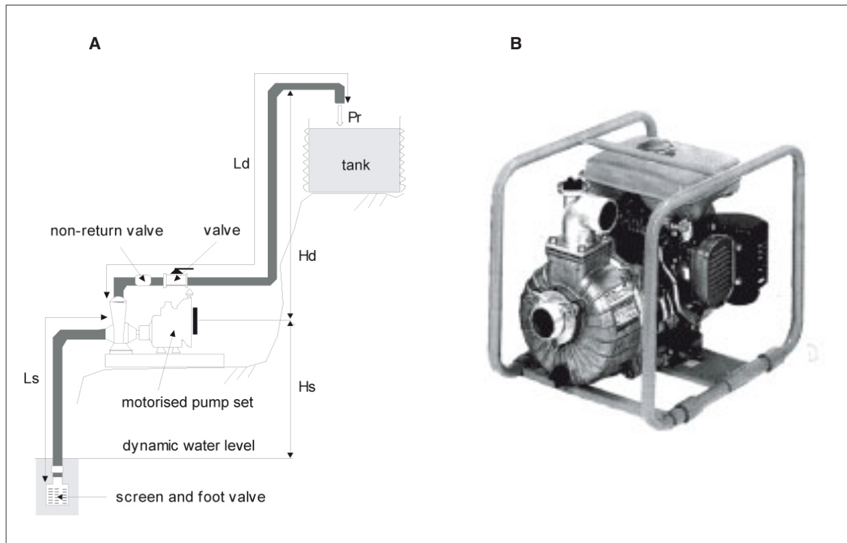
Figure 9.13: Surface-mounted motorised pump. A: installation diagram. B: photograph.
