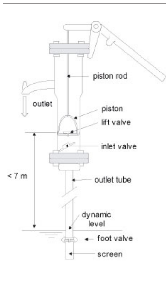
Figure 9.32: VN6-type suction pump.
