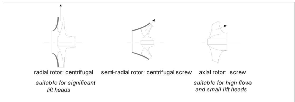
Figure 9.2: Rotor designs in turbopumps.
