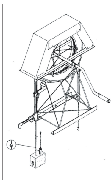
Figure 9.38: Rope pump.
