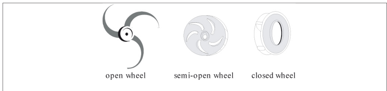
Figure 9.3: Rotor designs in centrifugal pumps.
