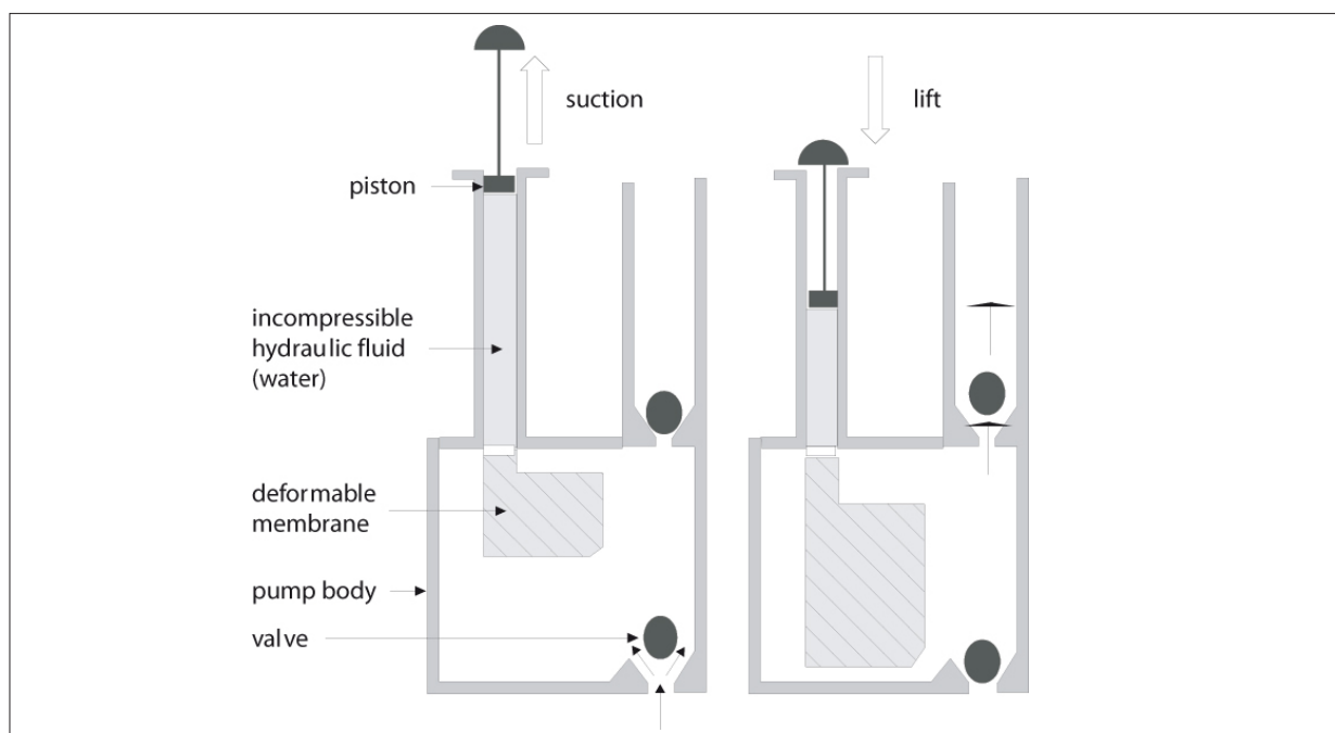
Figure 9.33: Working principle of Vergnet hydropump.
