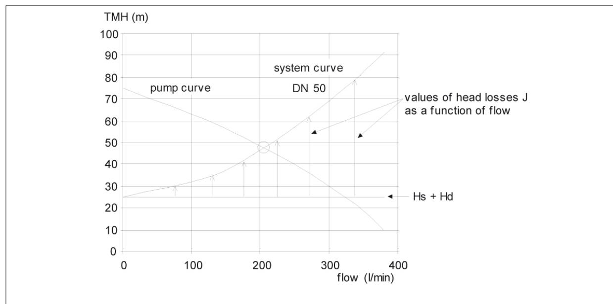
Figure 9.6: Working point (TEF2-50 pump in pipe system).
