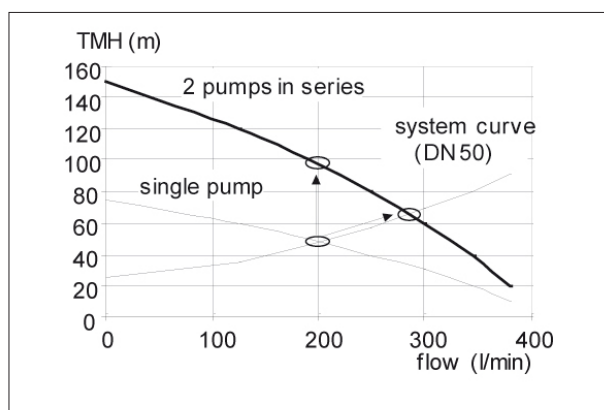
Figure 9.9: Characteristic curves for a single pump and for two pumps in series.
