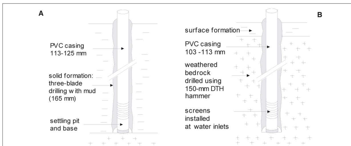
Figure 8.9: Rotary drilling (A) and DTH hammer (B).
