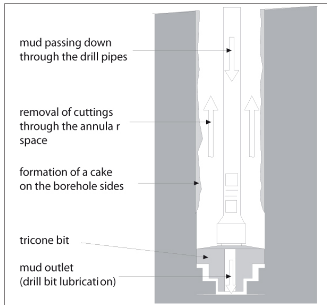
Figure 8.1: Working principle of rotary drilling.
