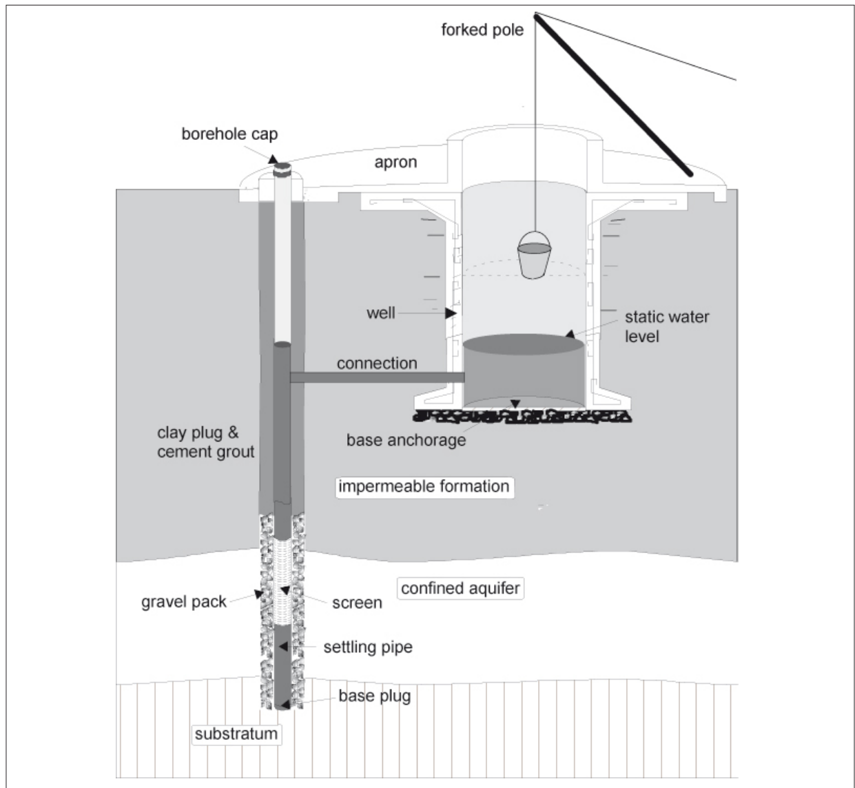
Figure 8.28: Lateral combined well (ACF, Mali, 2003).
