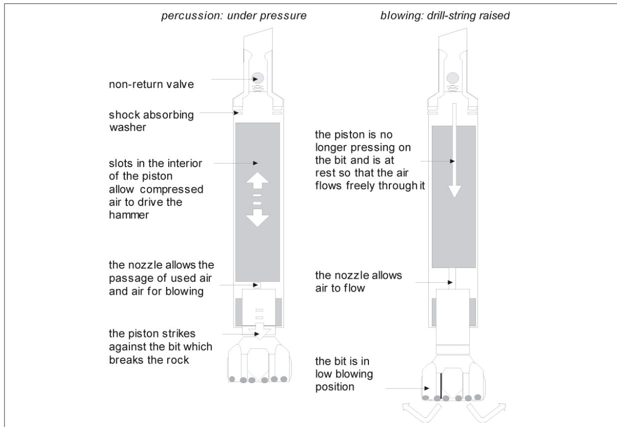
Figure 8.20: Hammer function.
