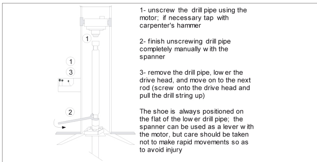
Figure 8.19: Removing a drill pipe.
