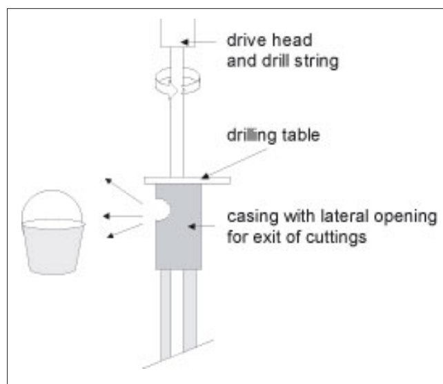
Figure 8.15: Collection of cuttings.
