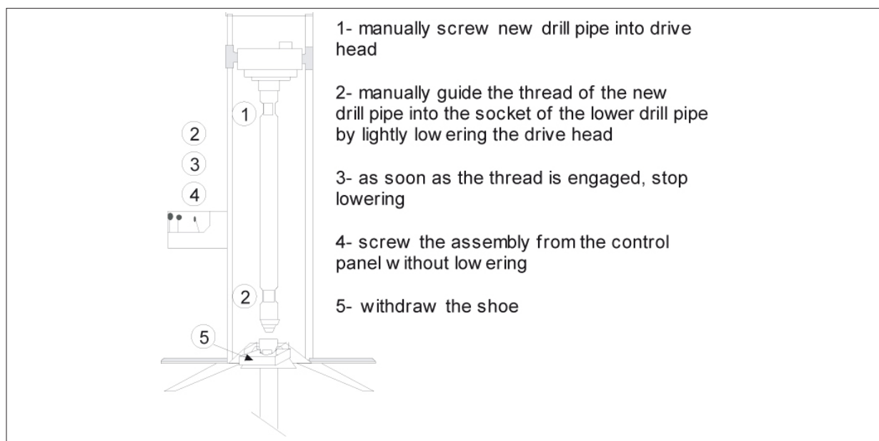
Figure 8.18: Locking drill pipes in suspension.
