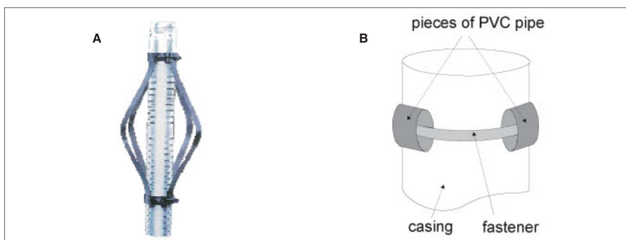
Figure 8.23 Centralisers.
