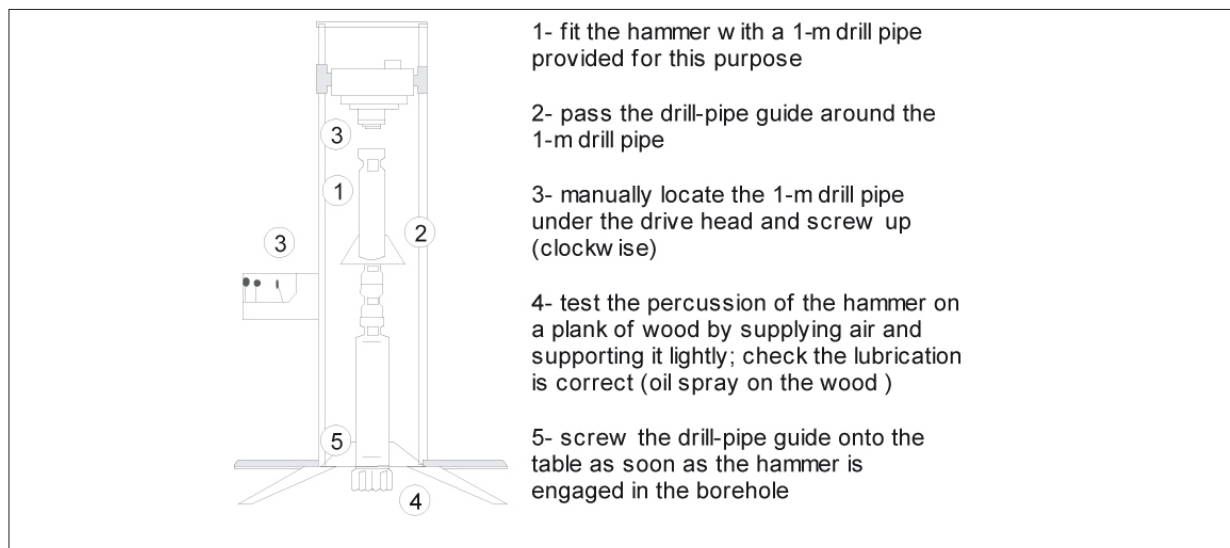
Figure 8.21: Fitting the hammer.
