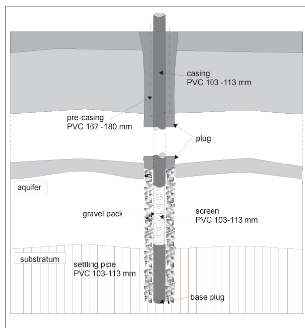
Figure 8.22: Borehole equipment (based on ACF, Uganda, 1997).
