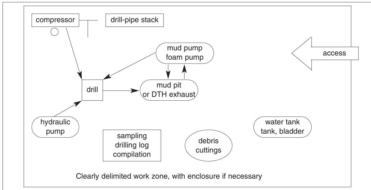
Figure 8.12: Site organisation.
