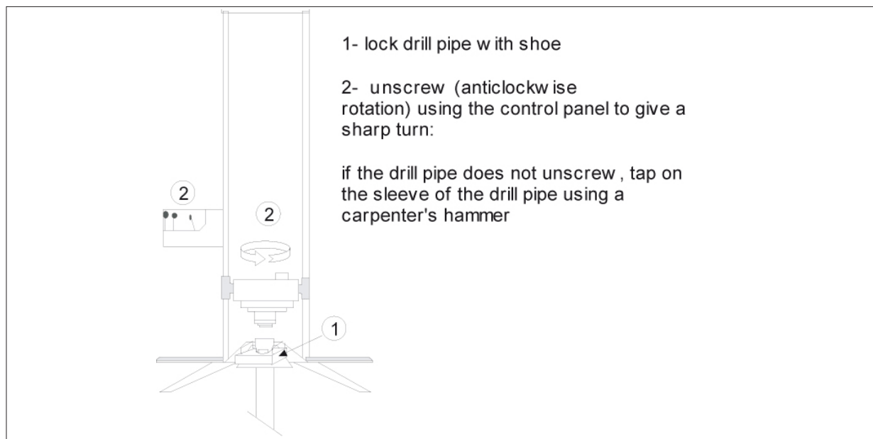
Figure 8.17: Unscrewing a drill pipe.
