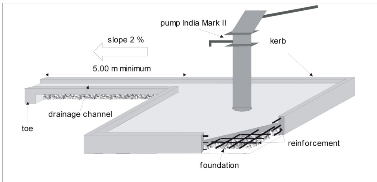
Figure 8.26: Borehole surface works (ACF, Kampala, Uganda, 1996).
