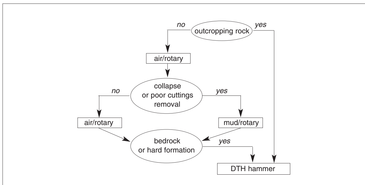
Figure 8.11: Flow chart for selection of drilling technique.
