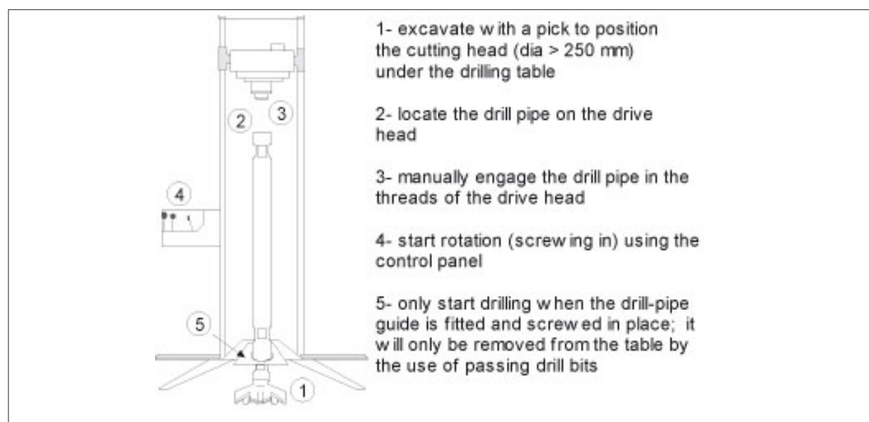
Figure 8.16: Fitting the first drill-pipe.
