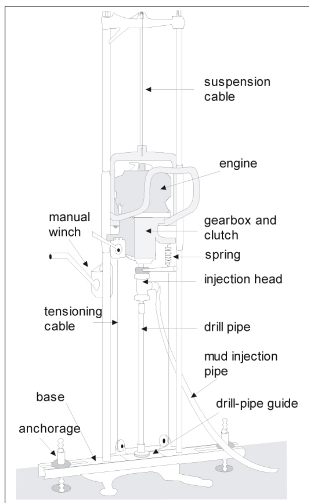
Figure 8.6: The ACF-PAT 201 drilling rig.
