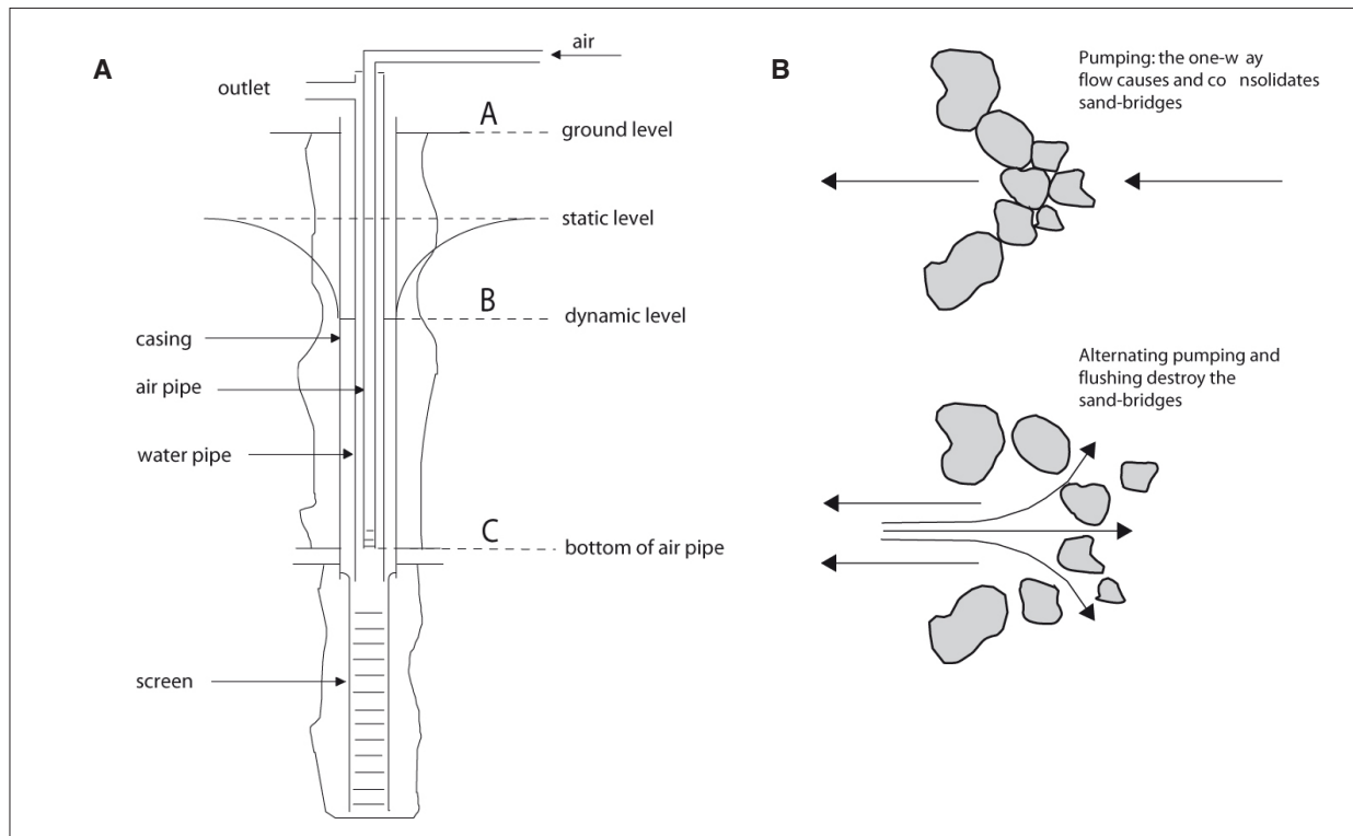
Figure 8.25: Air-lift. A: design. B: sand-bridge destruction.
