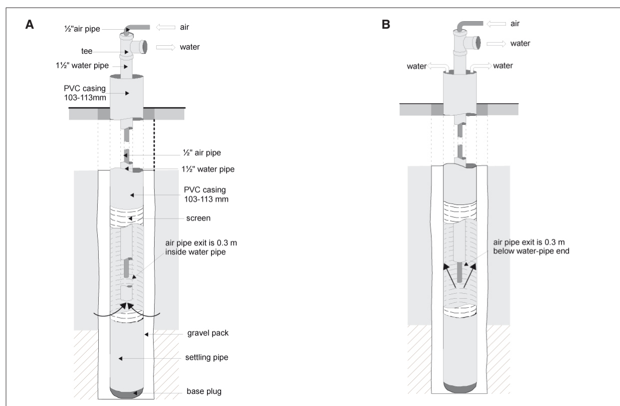
Figure 8.24: Air-lift development. A: pumping phase. B: blowing phase.
