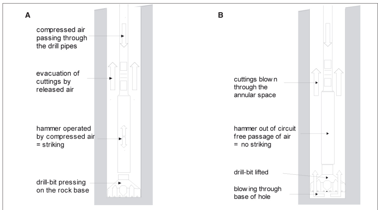
Figure 8.2: Working principle of DTH hammer drilling.
