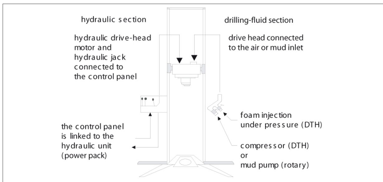
Figure 8.7: The ACF-PAT 301 drilling rig – working principle.
