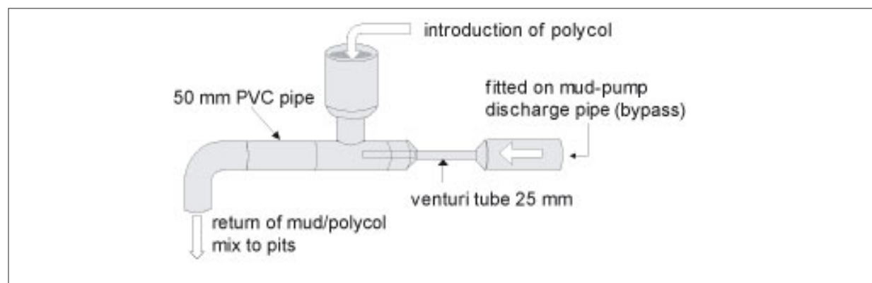
Figure 8.14: Venturi mixer made from PVC fittings.
