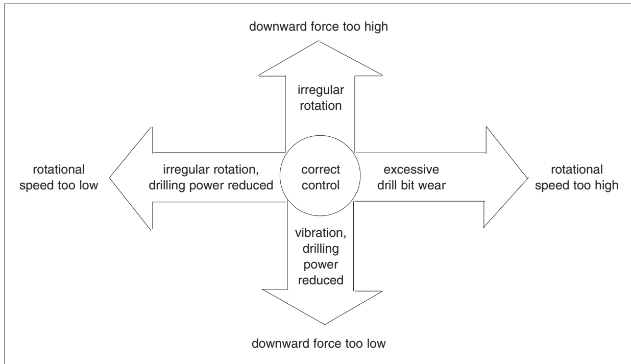
Figure 8.3: Control of downward force and rotation.
