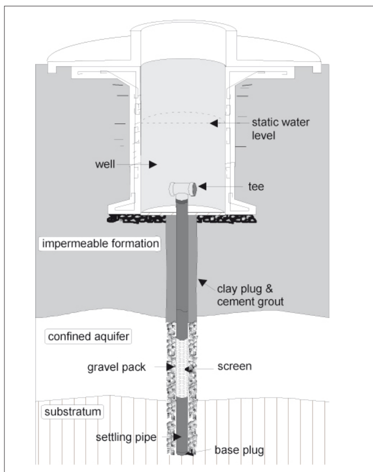
Figure 8.27: Central combined well (ACF, Cambodia, 1998).
