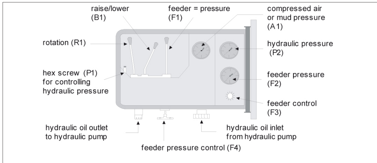
Figure 8.8: Control panel functions on the ACF-PAT 301 (1996 model).
