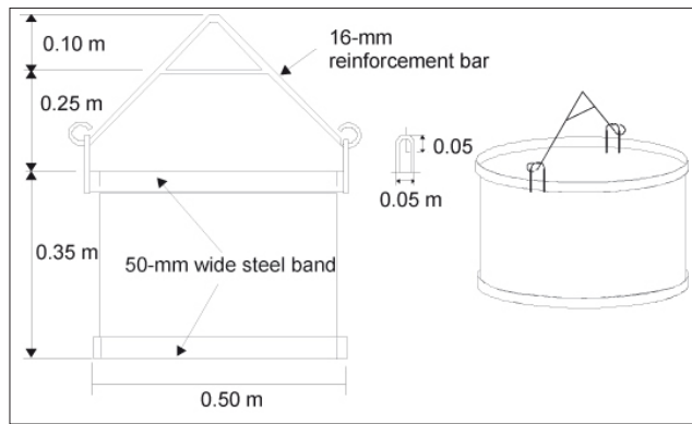
Figure 7.14: A bailer.
