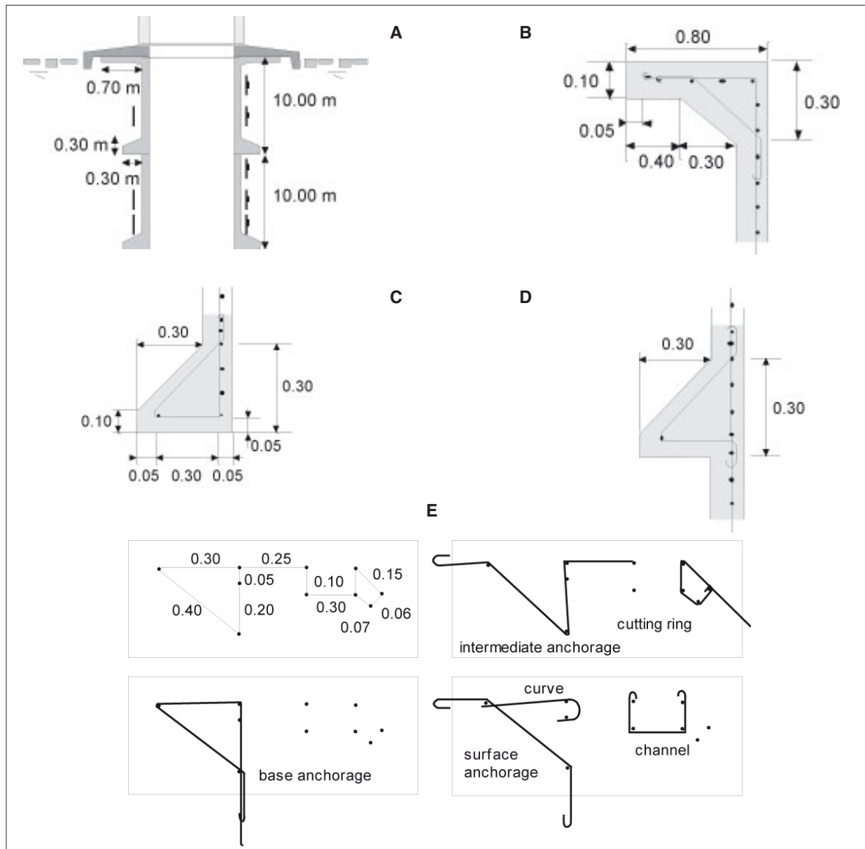
Figure 7.10: Reinforcement for lining anchorages.
