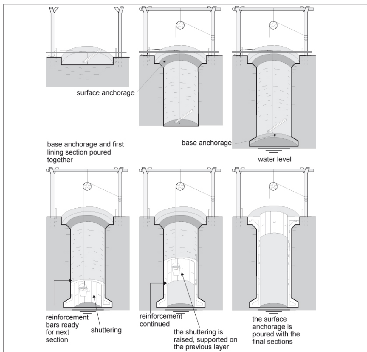
Figure 7.6: Bottom-up lining.
