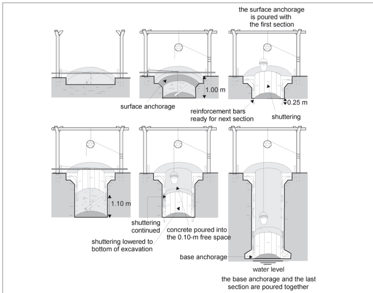
Figure 7.7: Top-down lining.
