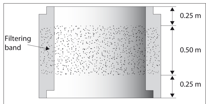
Figure 7.9: Filtering concrete ring.
