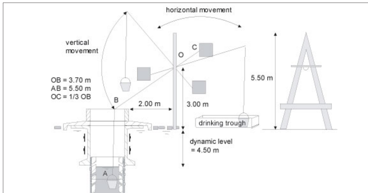
Figure 1: Shaduf.
