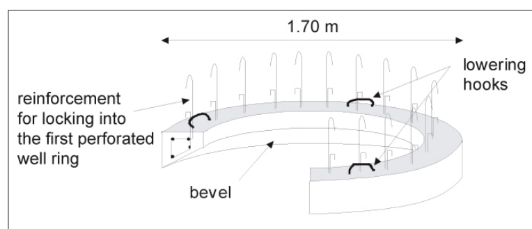
Figure 7.12: Cutting ring 1.4 / 1.6 m diameter.
