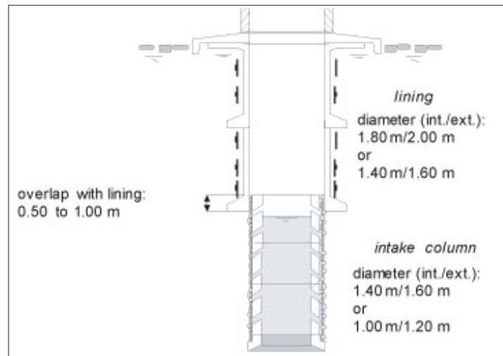
Figure 7.3: Lined well with independent intake.
