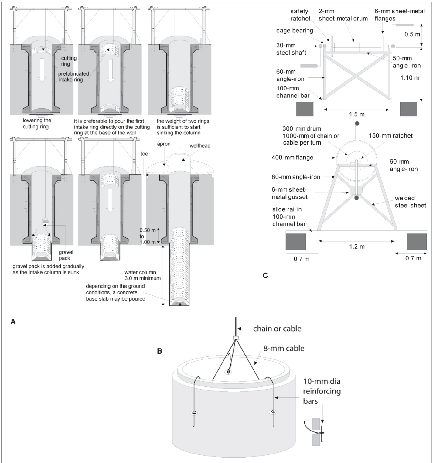
Figure 7.13: Sinking an independent intake.
