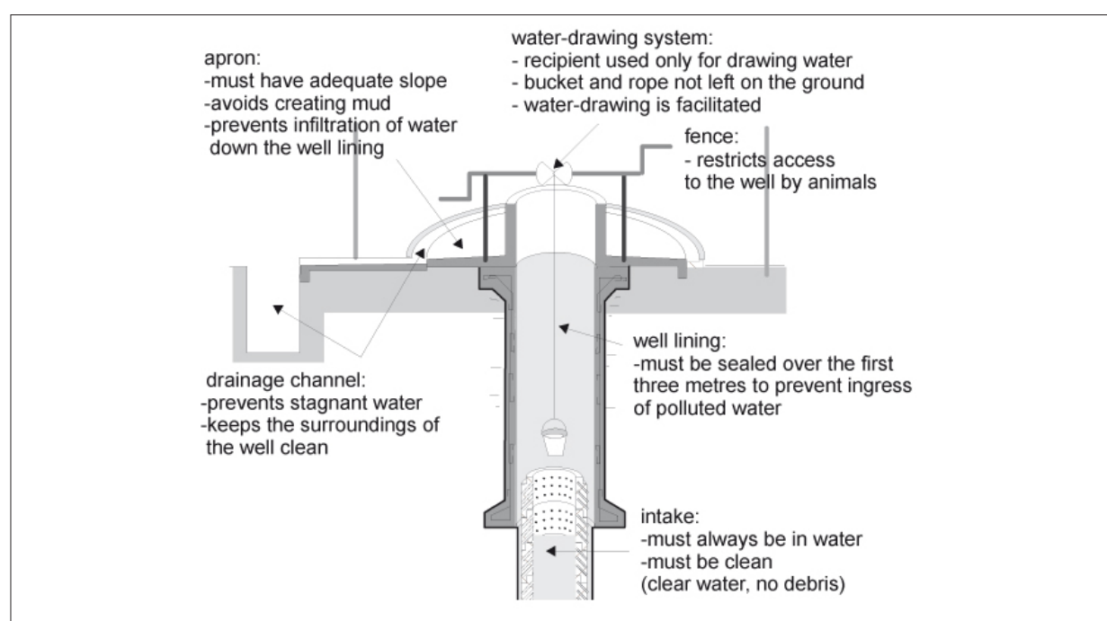
Figure 7.15: Protecting a well from pollution.
