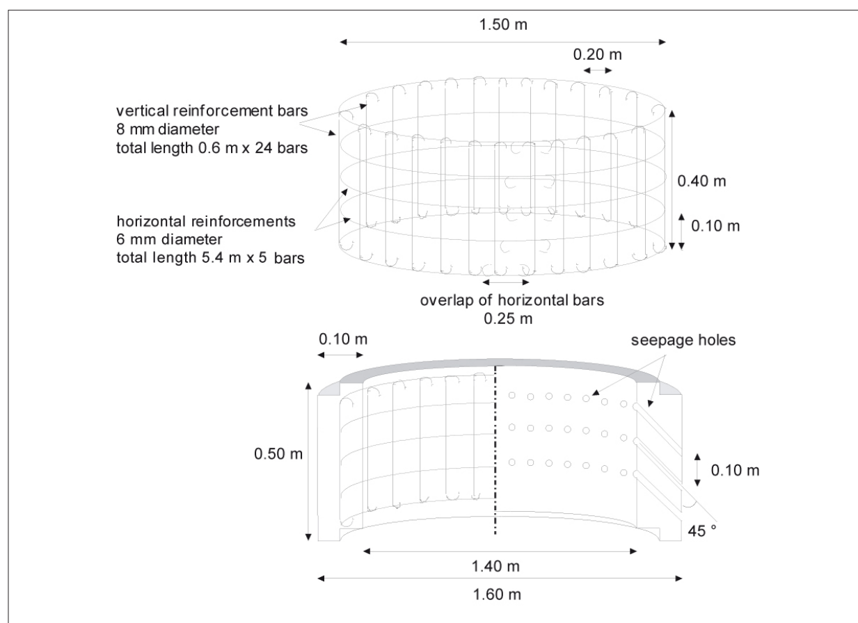
Figure 7.11: Reinforcement of perforated rings.
