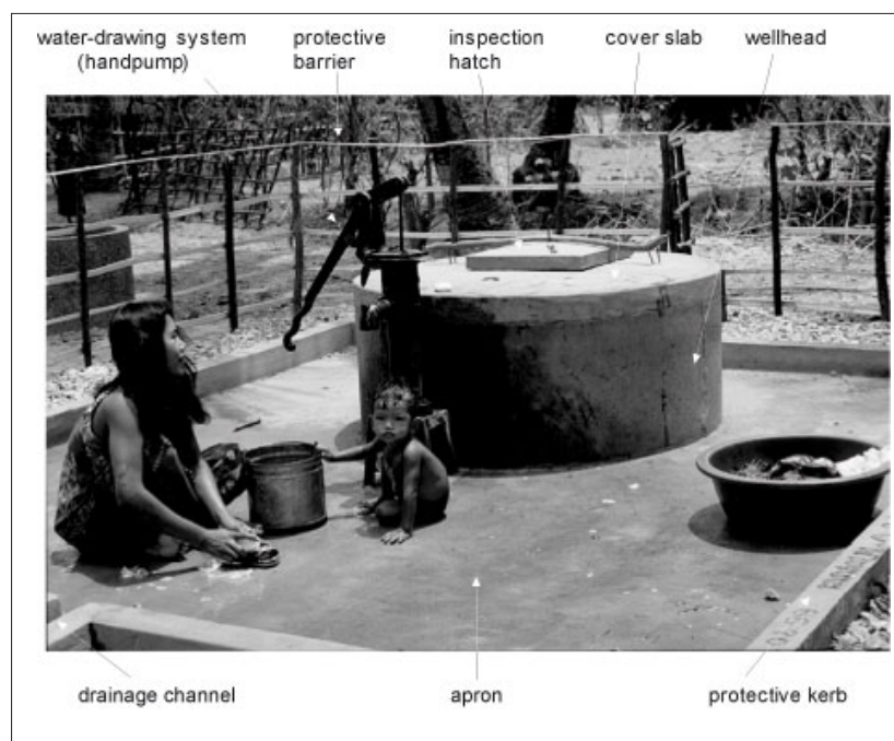
Figure 7.1: Well surface works (ACF, Cambodia, 1998).
