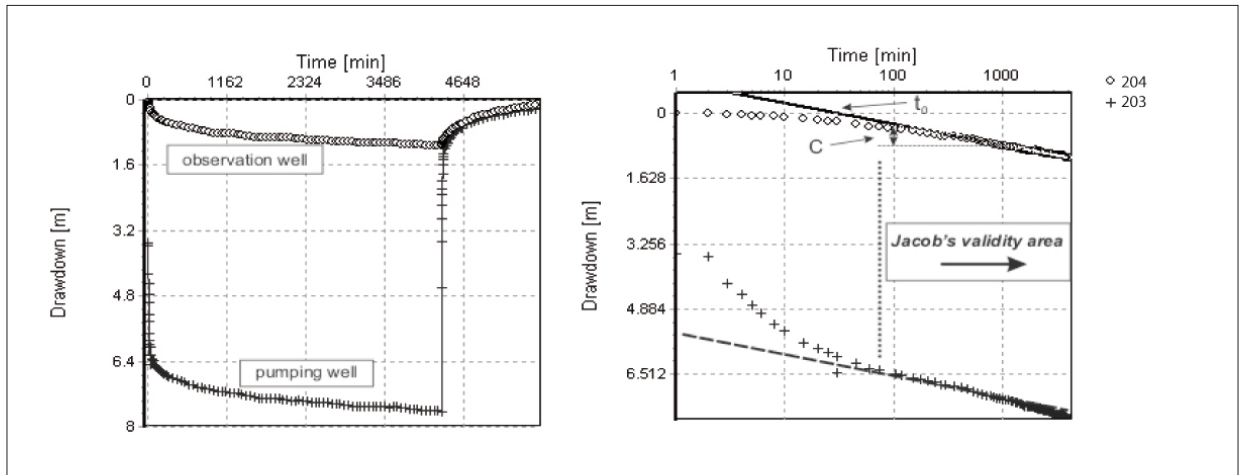
Figure 6.3: Aquifer-test interpretation using Jacob's method.
