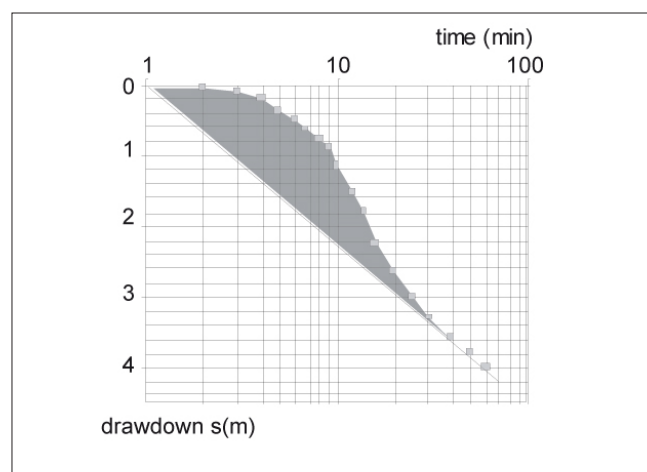
Figure 6.20: Capacity effect (drawdown delay).
