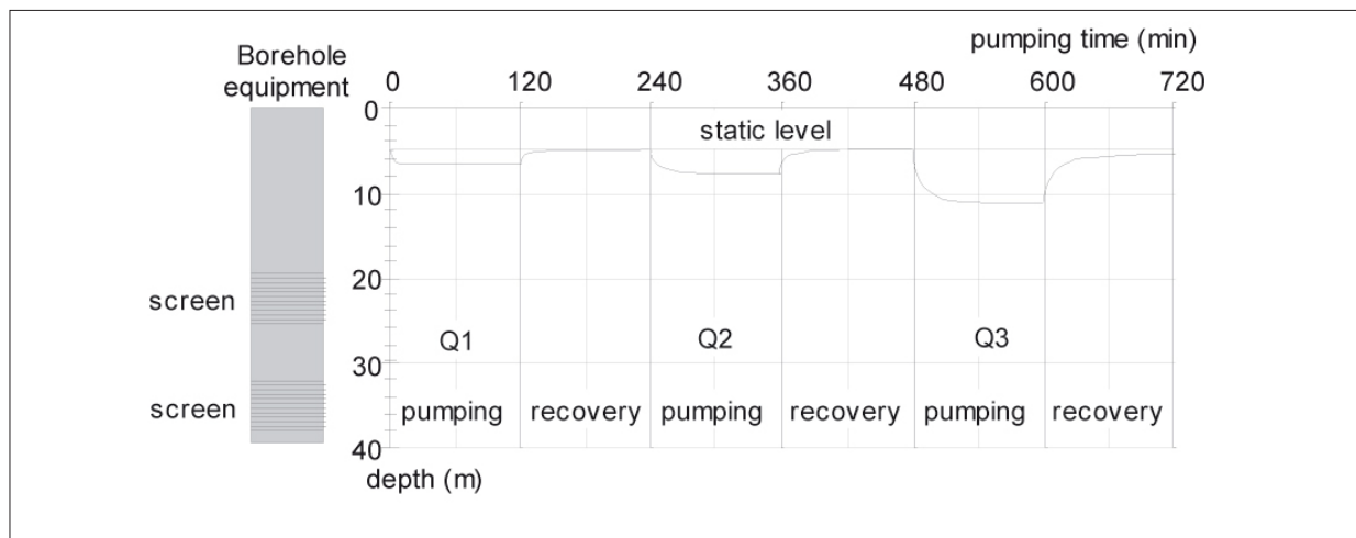
Figure 6.11: Water level as a function of time.
