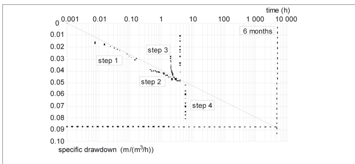
Figure 6.18: Extrapolation of specific drawdown, well P1.
