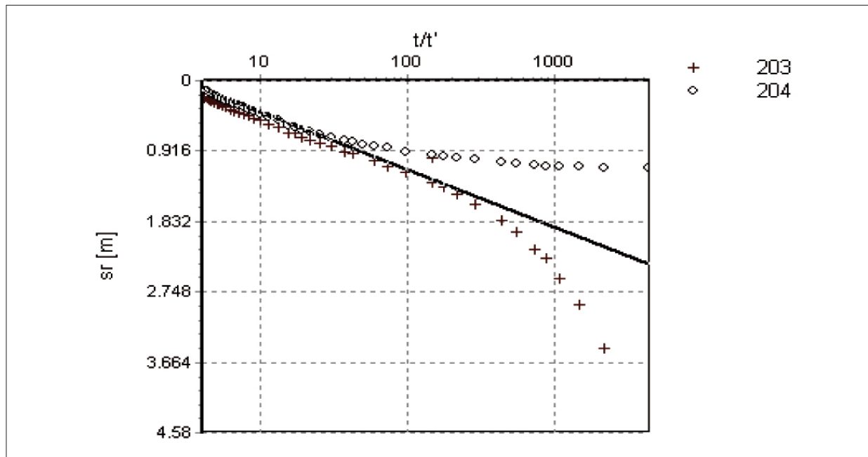
Figure 6.4: Aquifer-test interpretation using Theis's recovery method.
