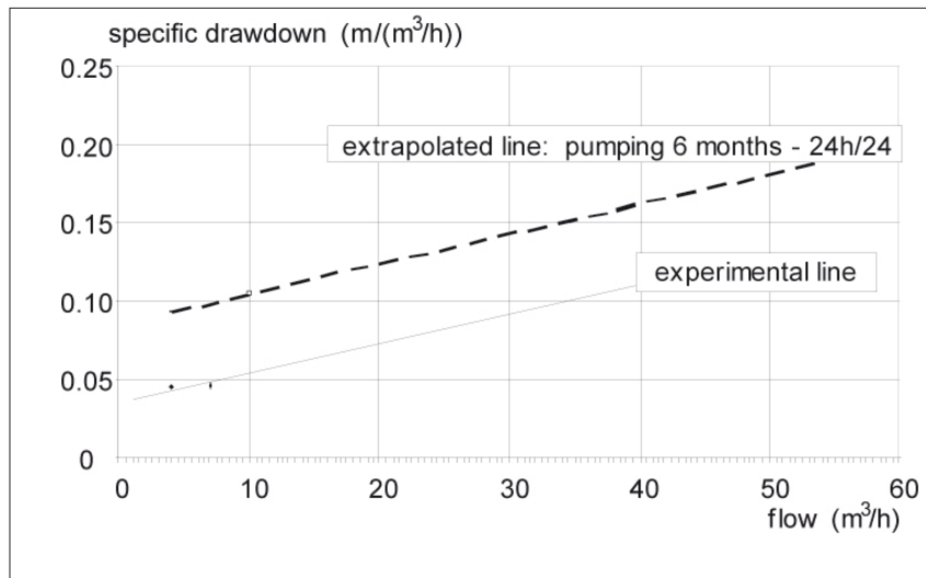
Figure 6.19: Extrapolation of drawdown, well P1.
