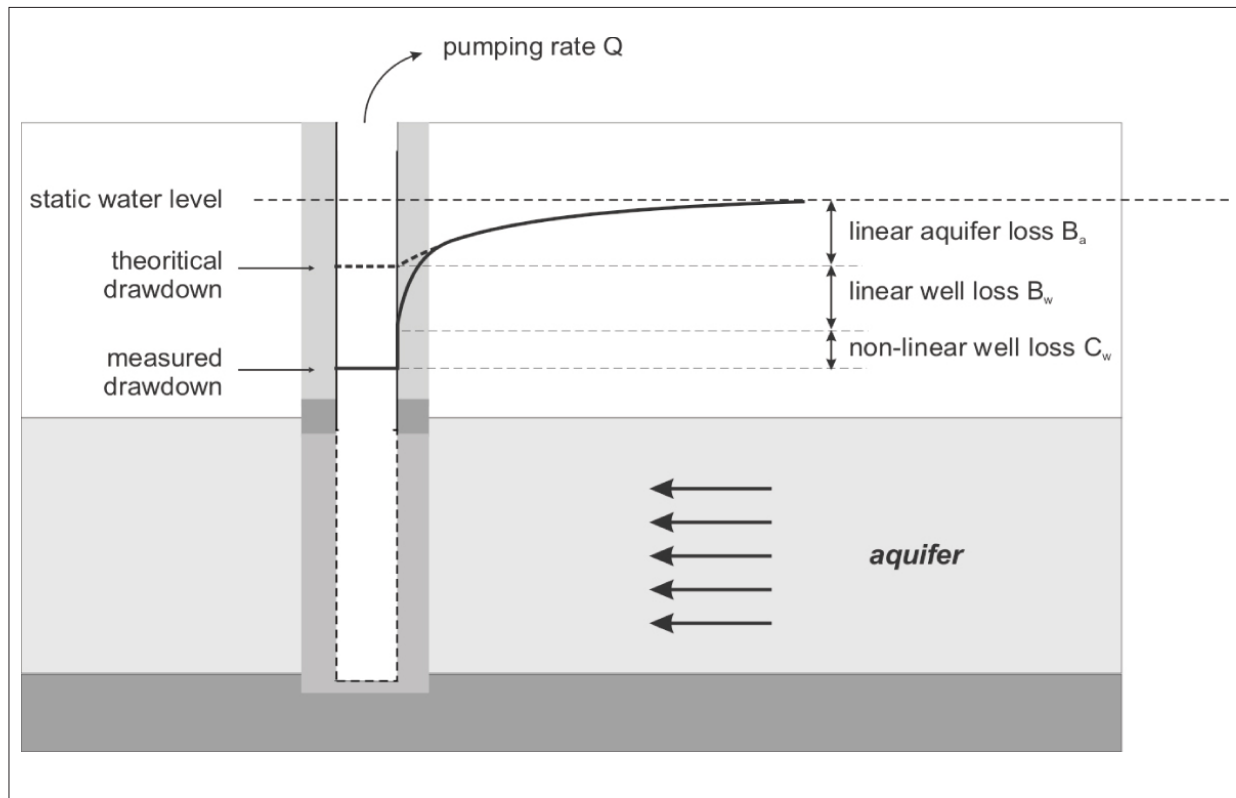
Figure 6.6: Various head-losses in a pumped well.
