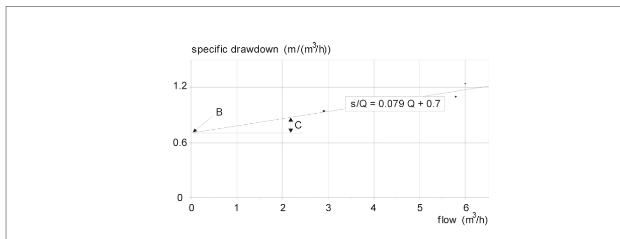
Figure 6.7: Calculation of head losses.
