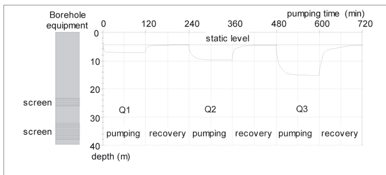
Figure 6.13: Water levels as a function of time.
