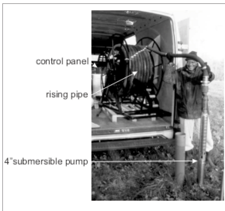
Figure 6.23: ACF pumping-test kit.
