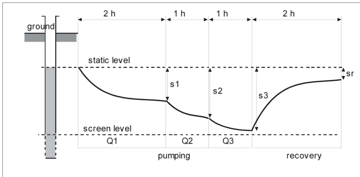
Figure 6.15: Well test in connected steps.
