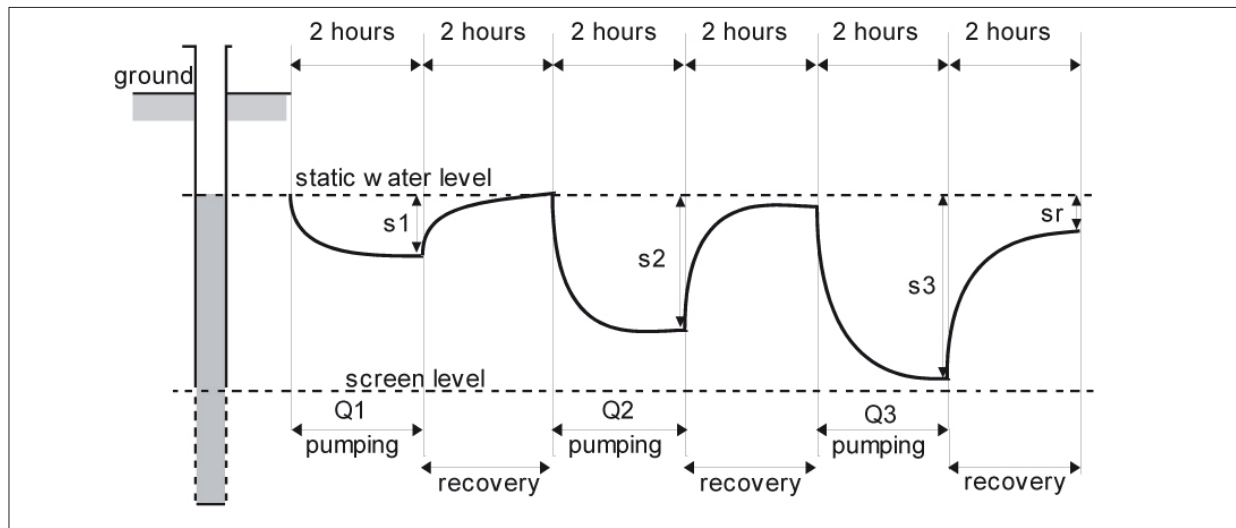
Figure 6.5: Well test with non-connected steps.
