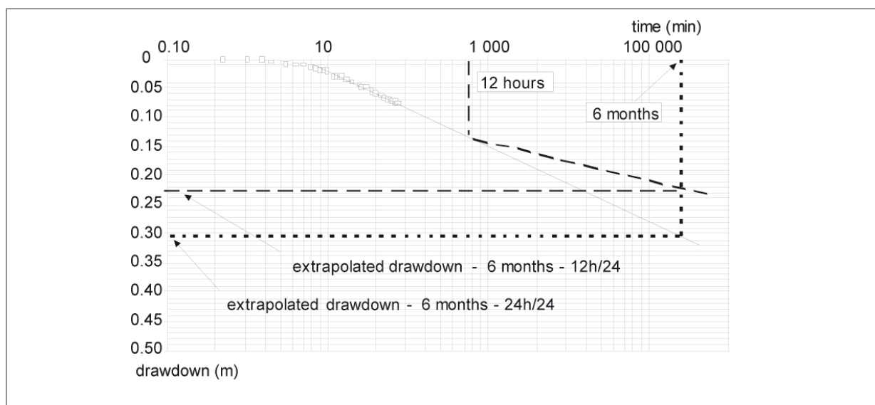
Figure 6.9: Extrapolation of drawdown as a function of time.
