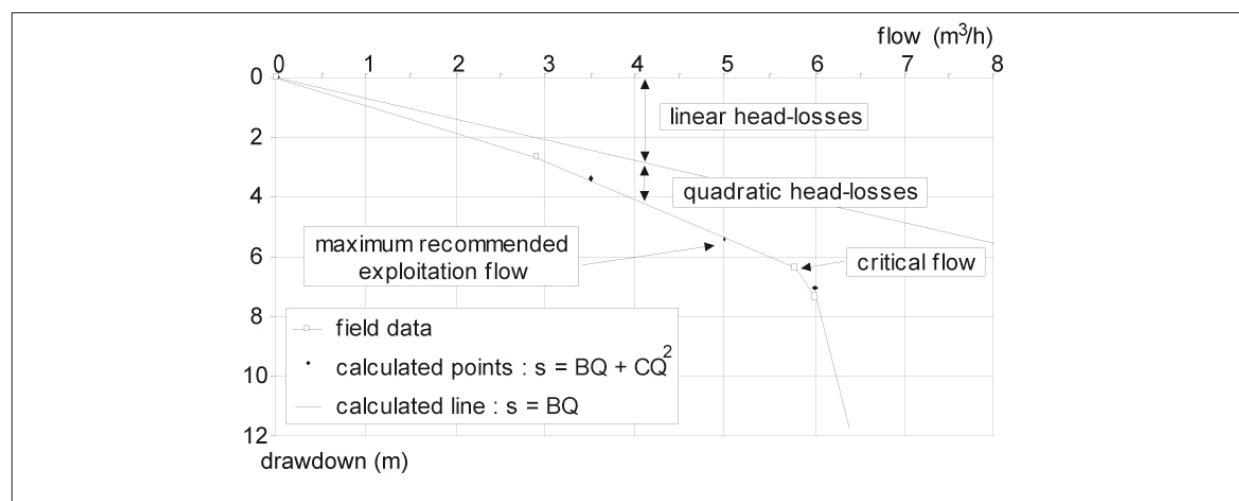
Figure 6.8: Well curve s = f(Q) of borehole F1.
