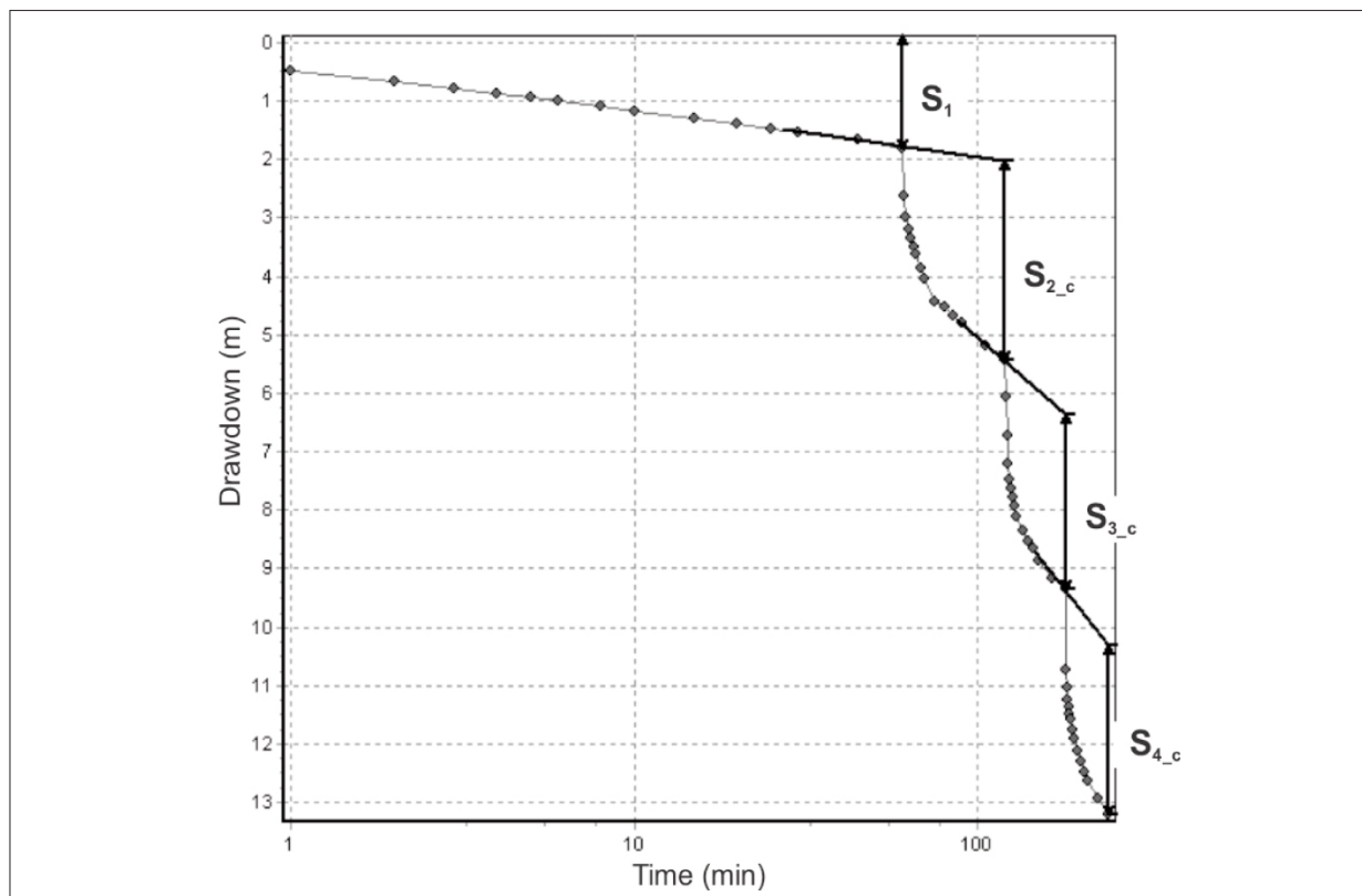
Figure 6.17: Graphical estimation of the corrected drawdown s_{i,C} , borehole 204.
