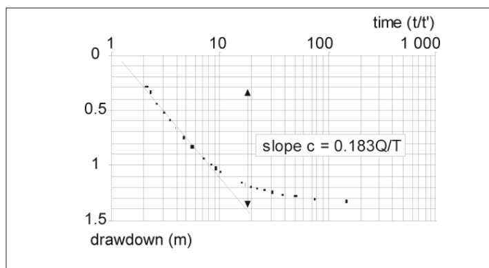
Figure 6.10: Recovery curve, borehole F4 – s = f(t/t') .
