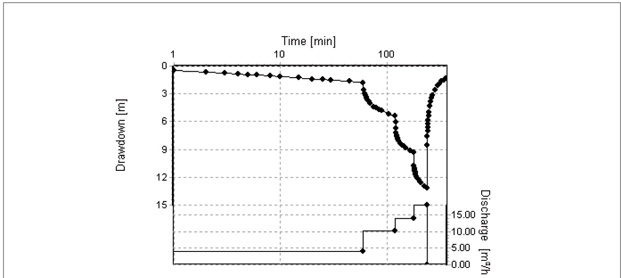
Figure 6.16: Four connected pumping steps, borehole 204.
