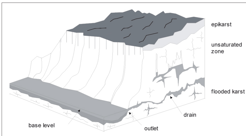
Figure 3.23: Karst.
