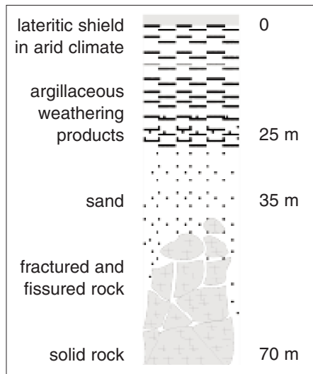
Figure 3.14: Weathering profile of granites.
