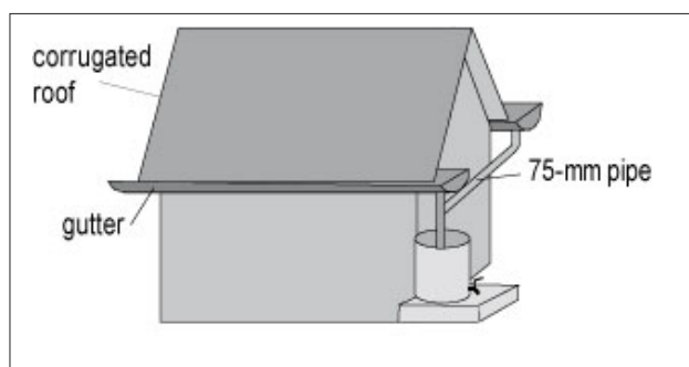
Figure 3.2: Harvesting of water from a roof.
