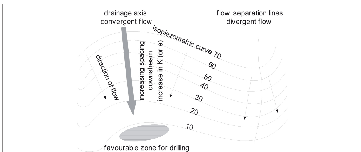
Figure 3.12: Piezometry.
