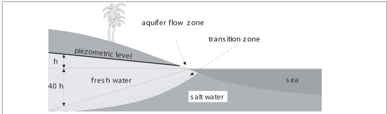
Figure 3.22: Saline wedge.
