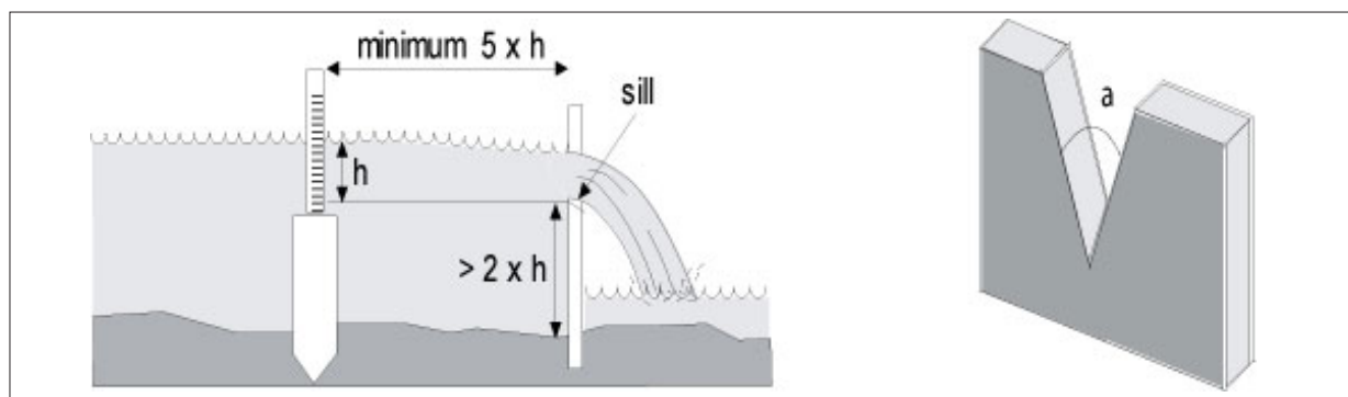
Figure 3.4: Thin-plate weir.
