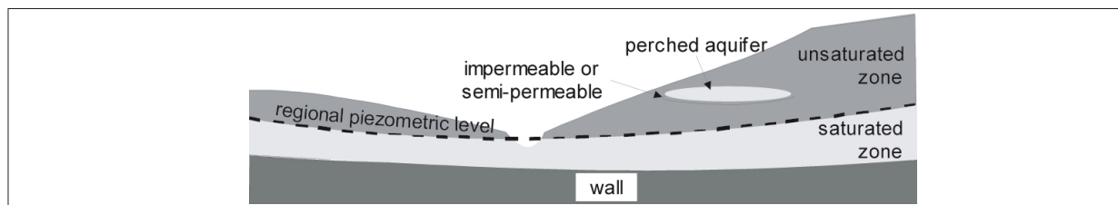
Figure 3.20: Perched aquifer.
