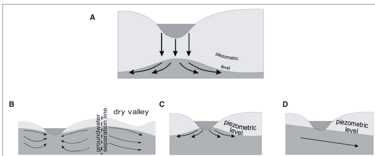
Figure 3.18: Relations between rivers and aquifers.
