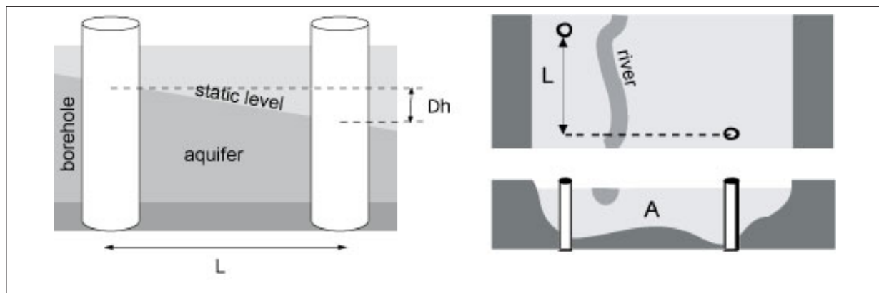
Figure 3.10: Application of Darcy's experiment.
