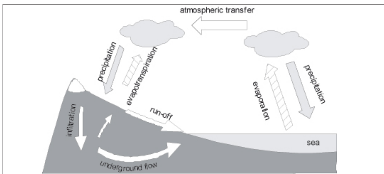
Figure 3.1: The water cycle.
