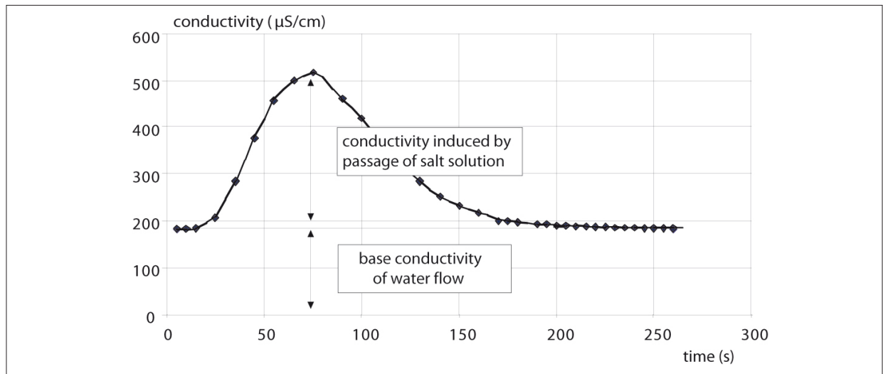
Figure 3.6: Salt-gulp method.
