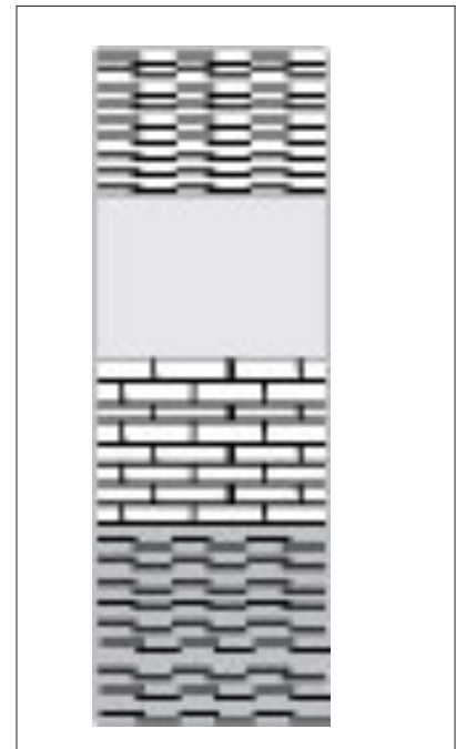
Figure 3.21: Stratified profile of a sedimentary basin.
