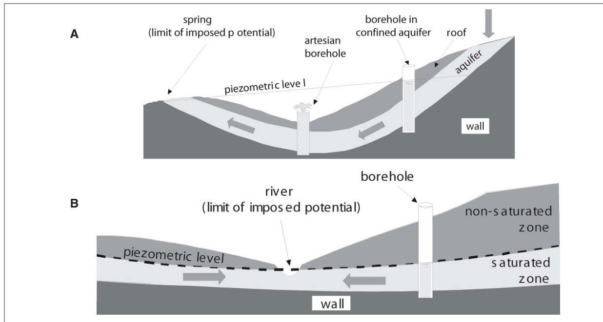
Figure 3.13: Aquifers. A: confined. B: unconfined.
