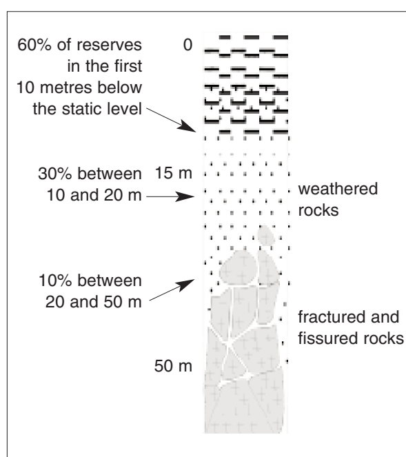
Figure 3.17 : Reserves in the bedrock zone.
