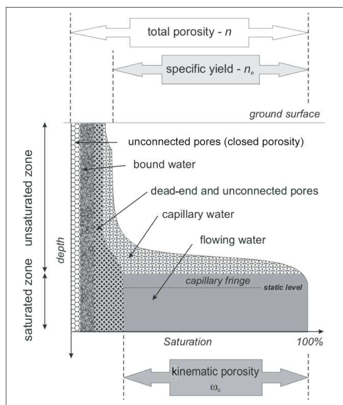
Figure 3.8: Groundwater type and storativity.
