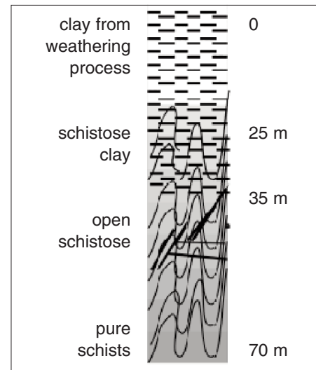
Figure 3.15: Weathering profile of schists.
