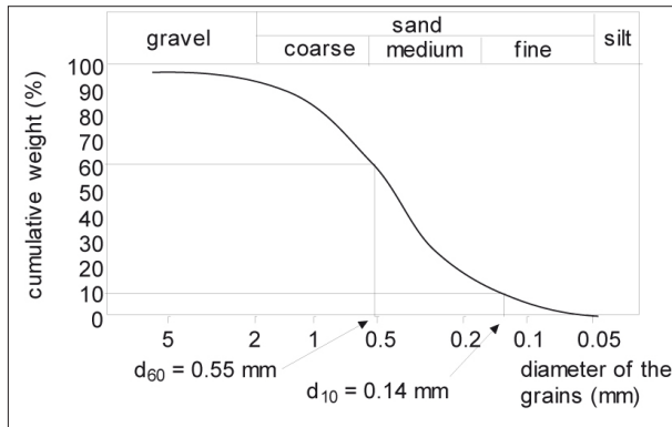
Figure 1: Particle-size curve.
