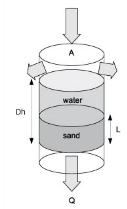
Figure 3.9: Darcy's experiment.
