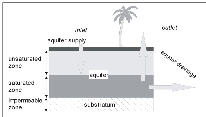
Figure 3.7: Storage and flow in an unconfined aquifer.
